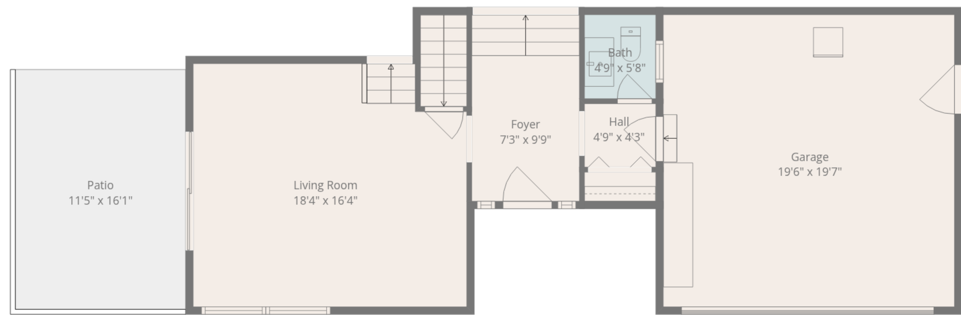
2nd Floor
