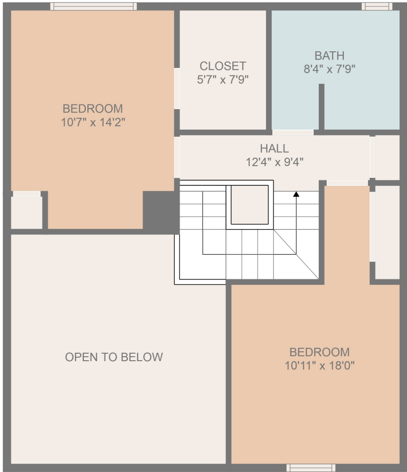
FLOOR 2
