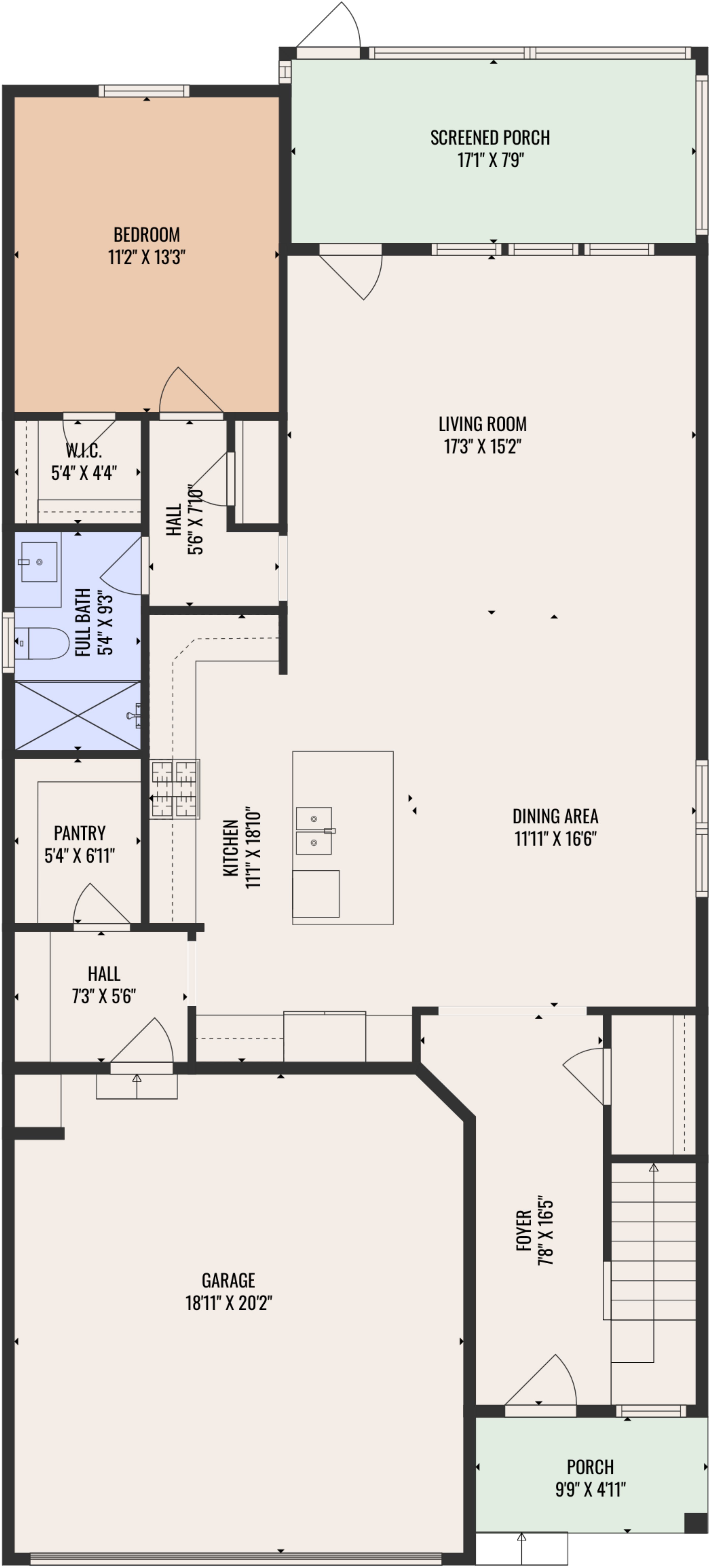
FLOOR 1
