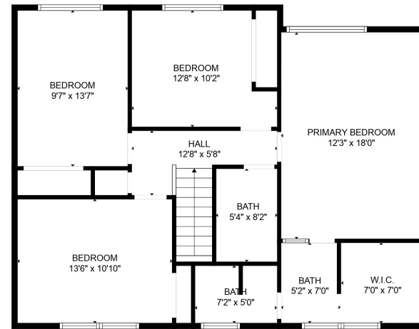
FLOOR 3
