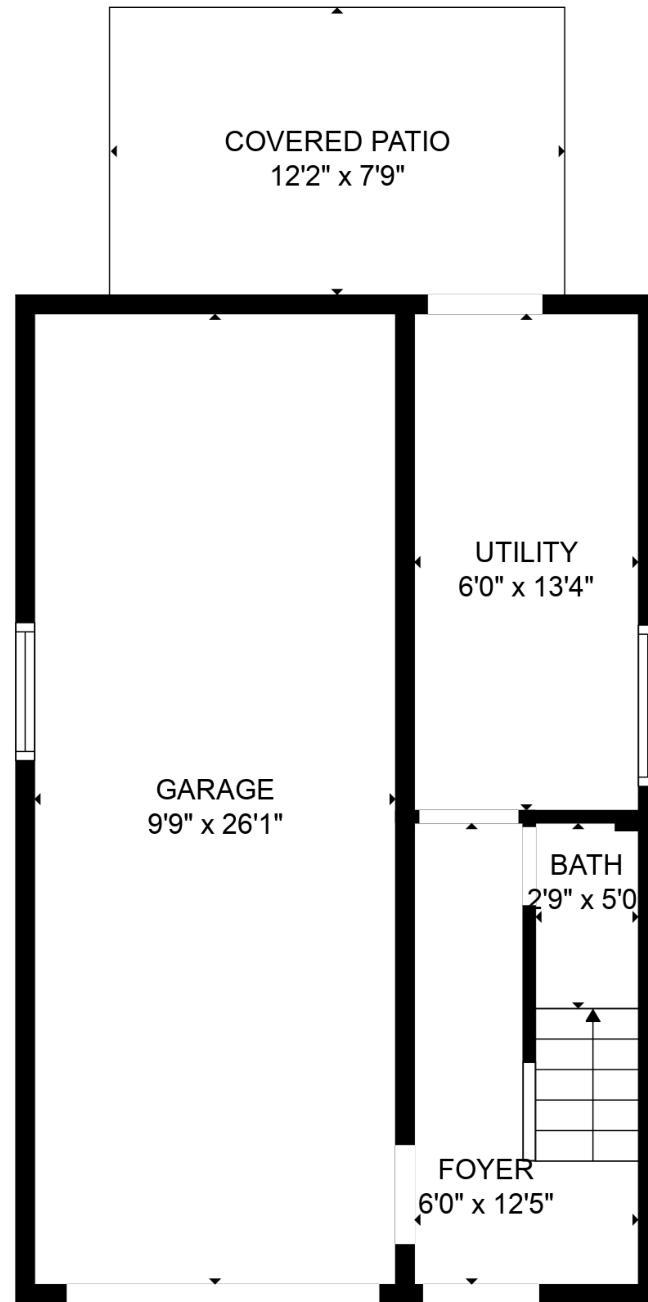
FLOOR 1
