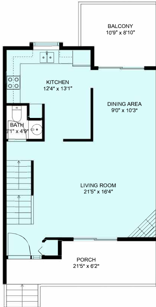
MAIN FLOOR
