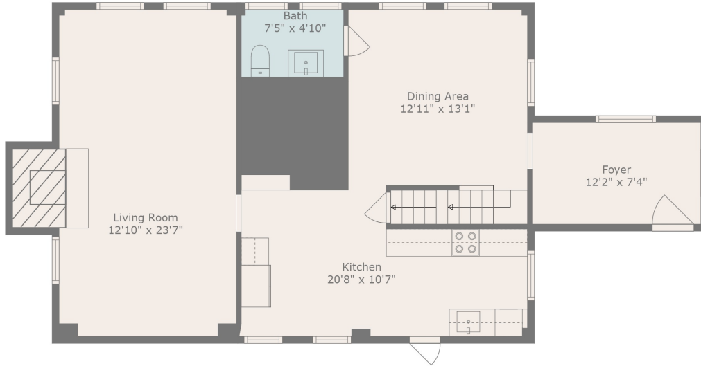
Floor 2
