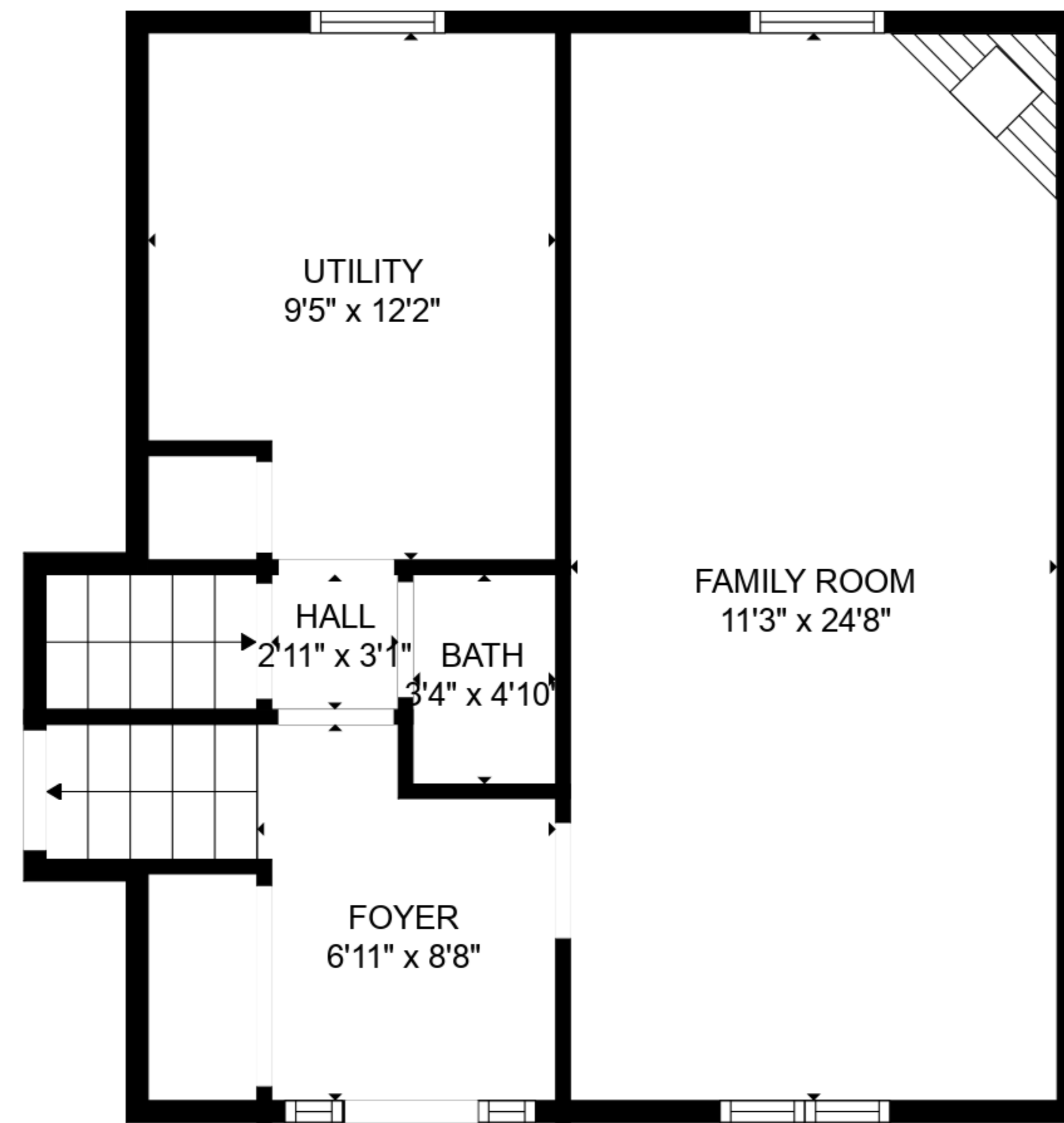
FLOOR 2
