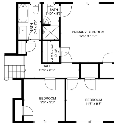
FLOOR 4
