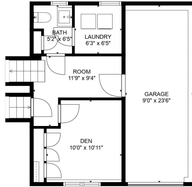
FLOOR 2
