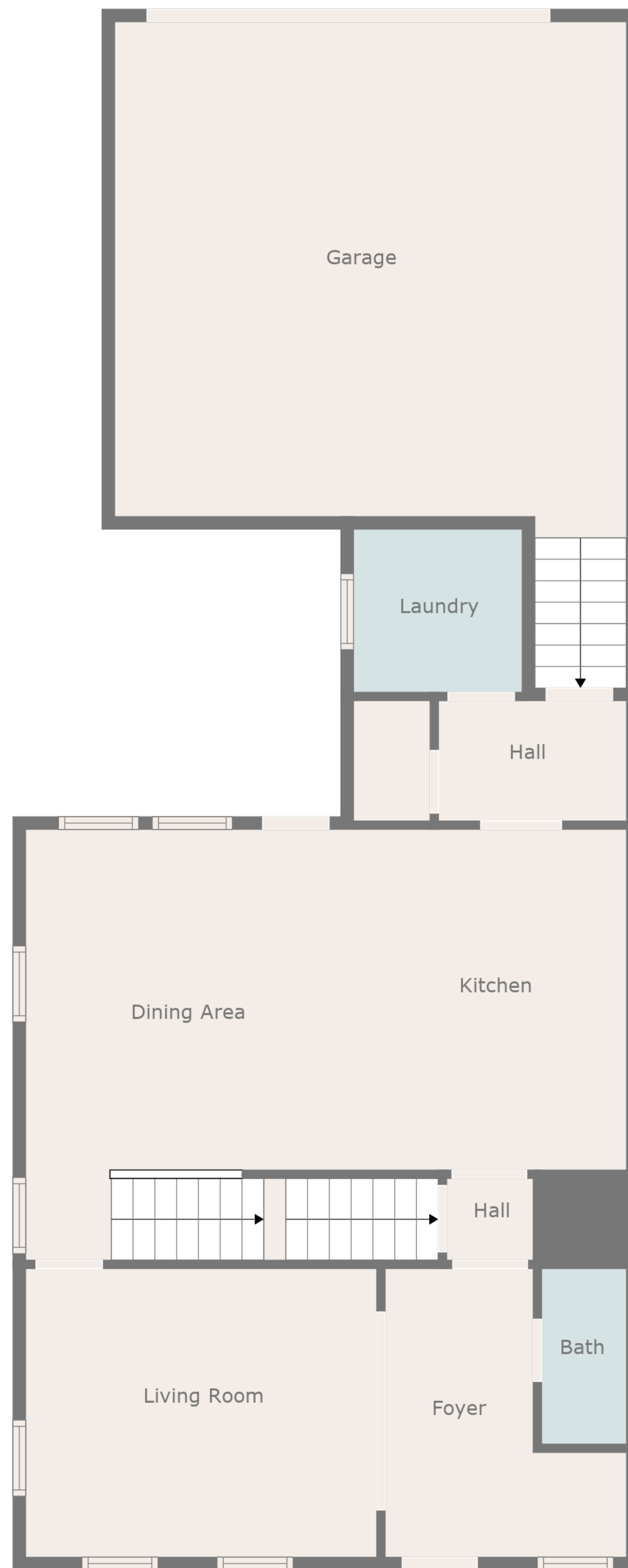
Floor 2
