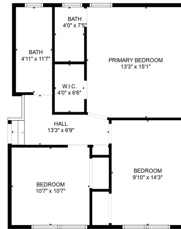
FLOOR 4
