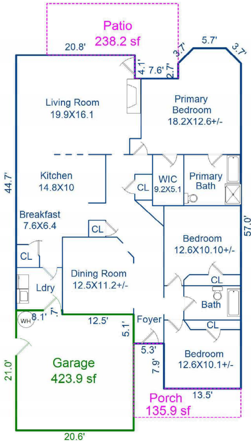
First Floor 1960.5 sf
