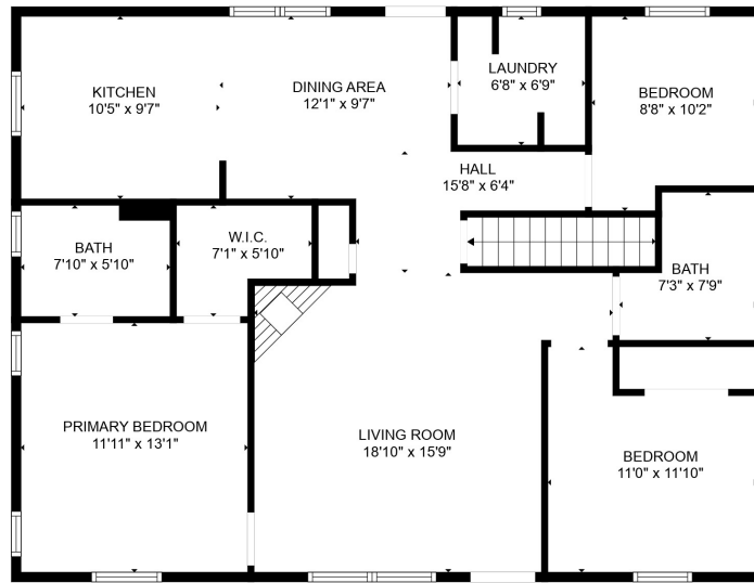
FLOOR 2
