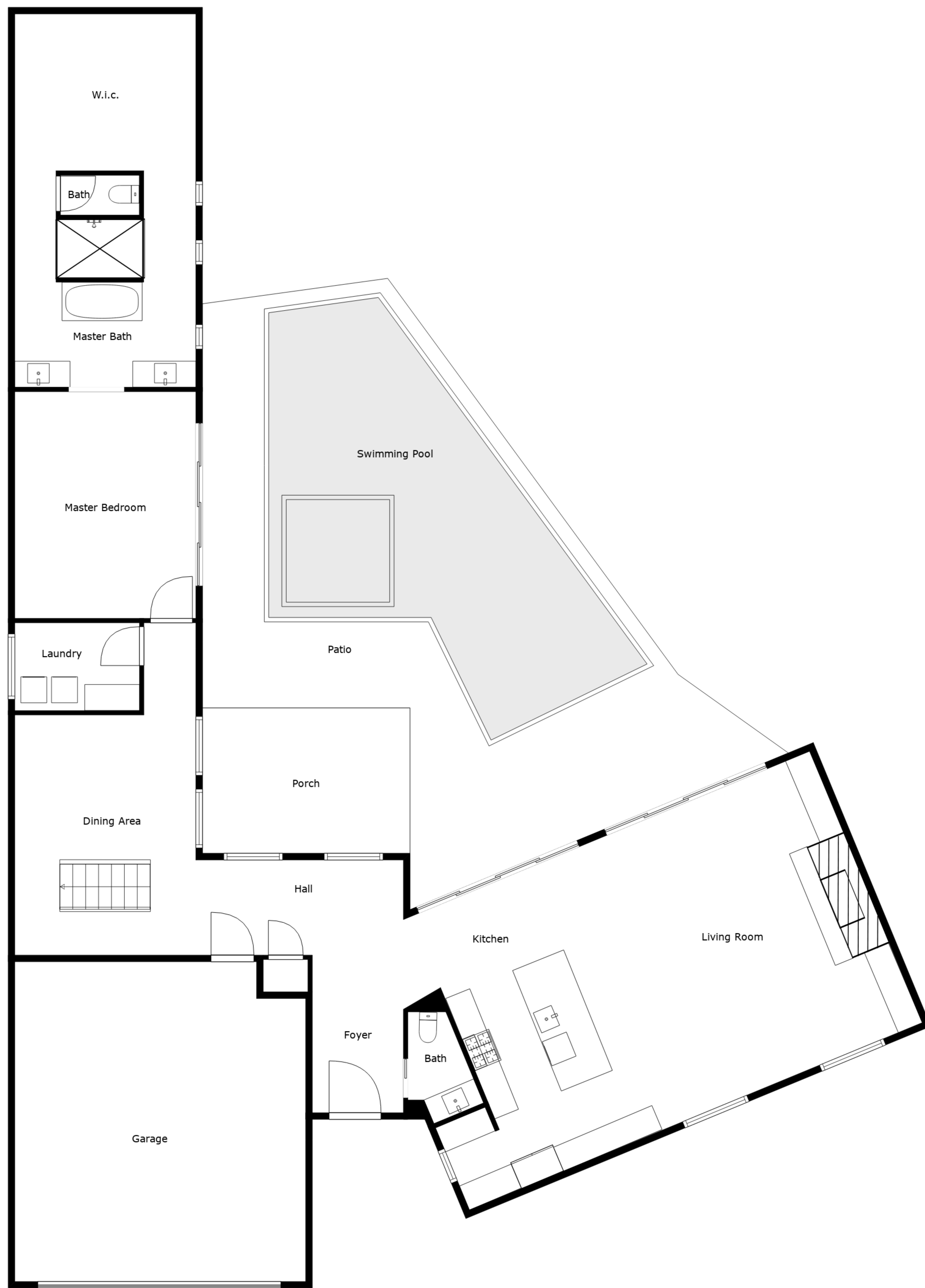
Floor 1
