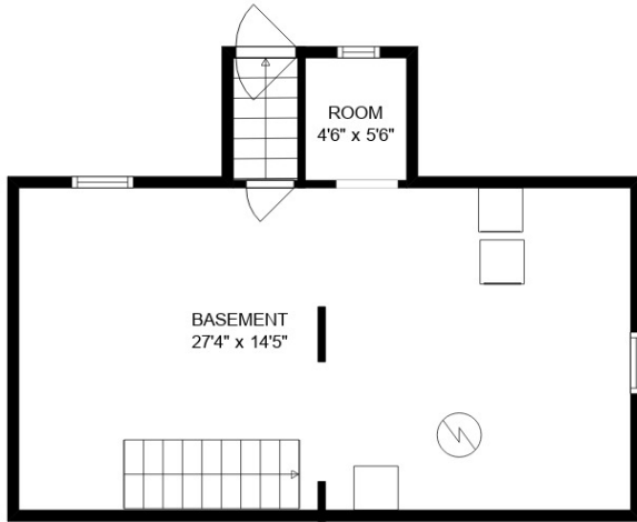
LOWER FLOOR
