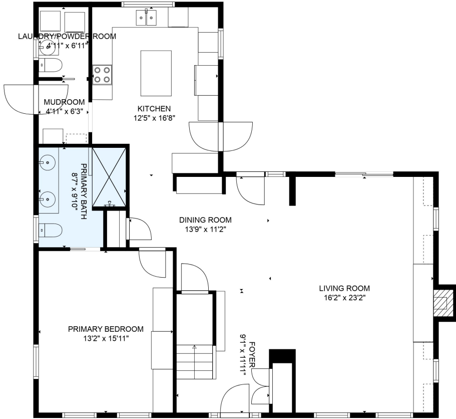
FLOOR 1
