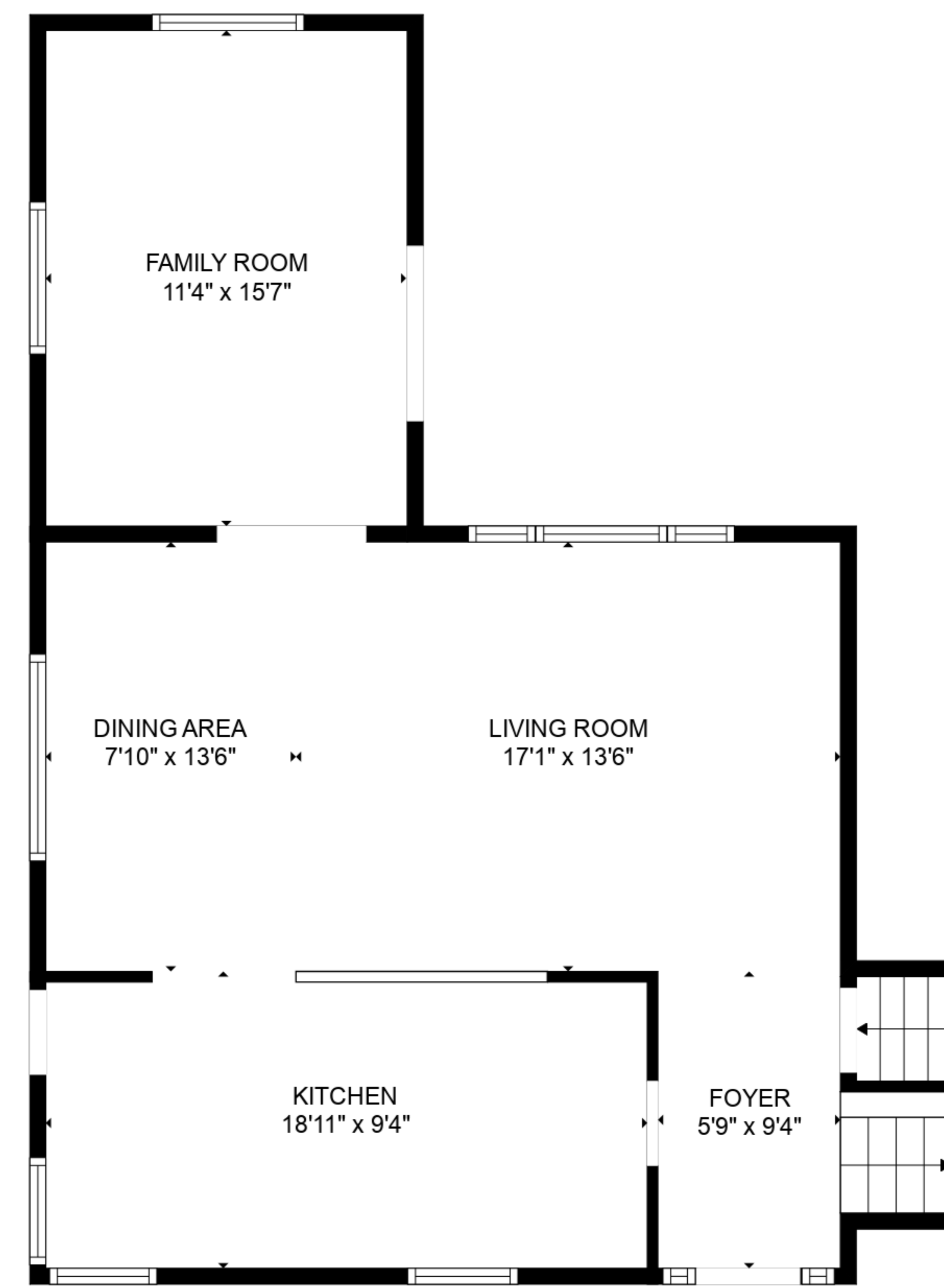
FLOOR 3
