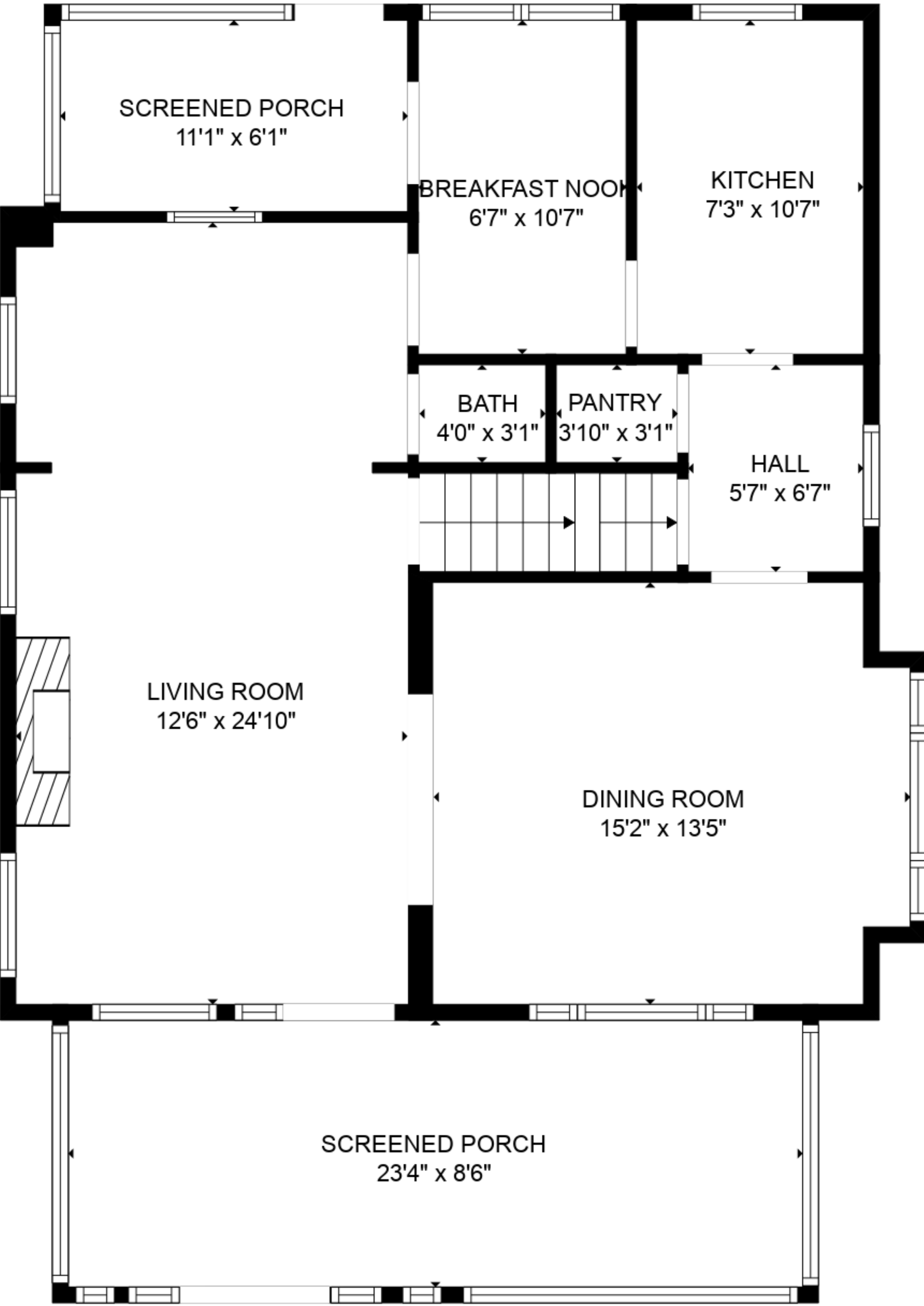
FLOOR 2
