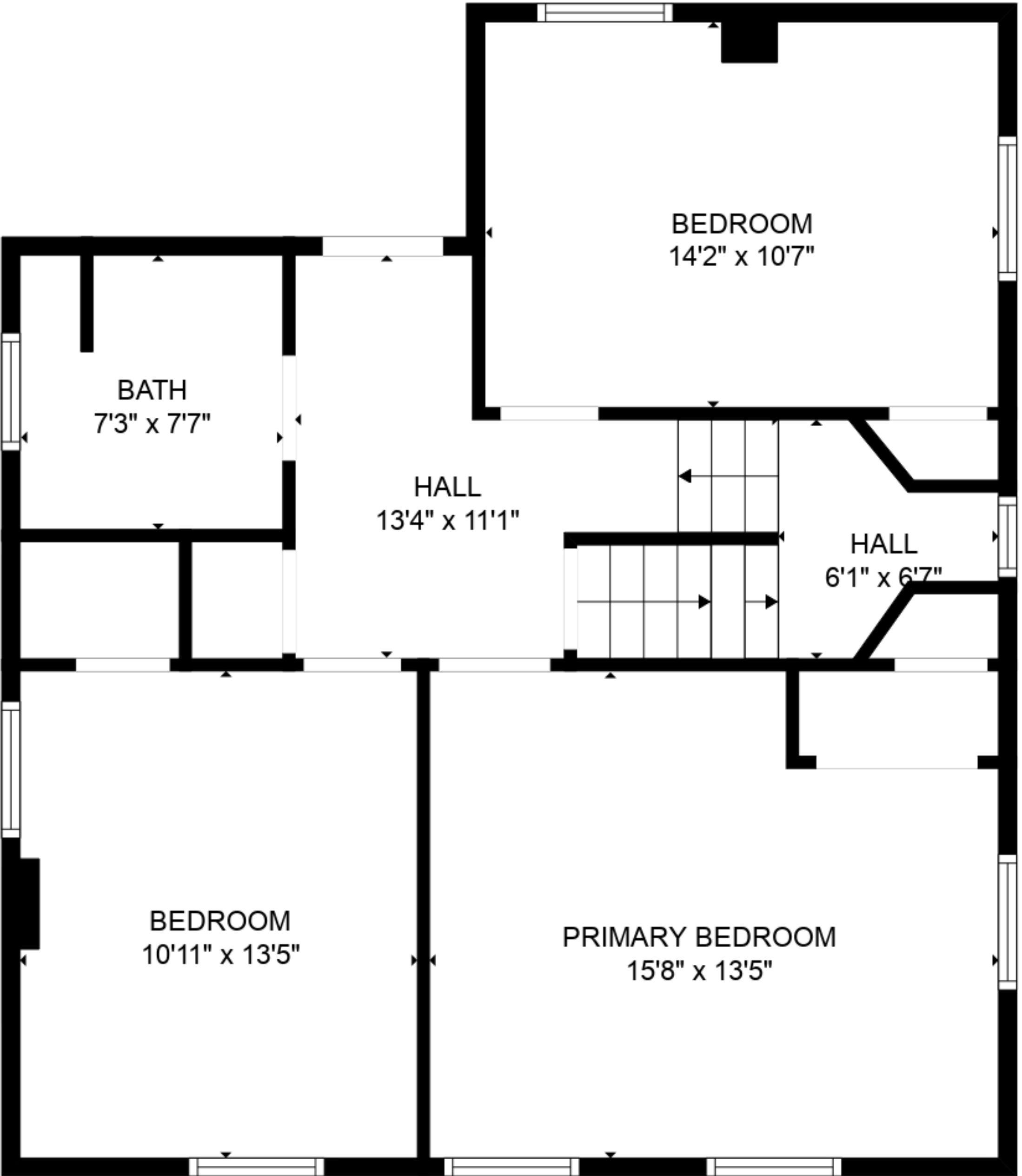
FLOOR 3
