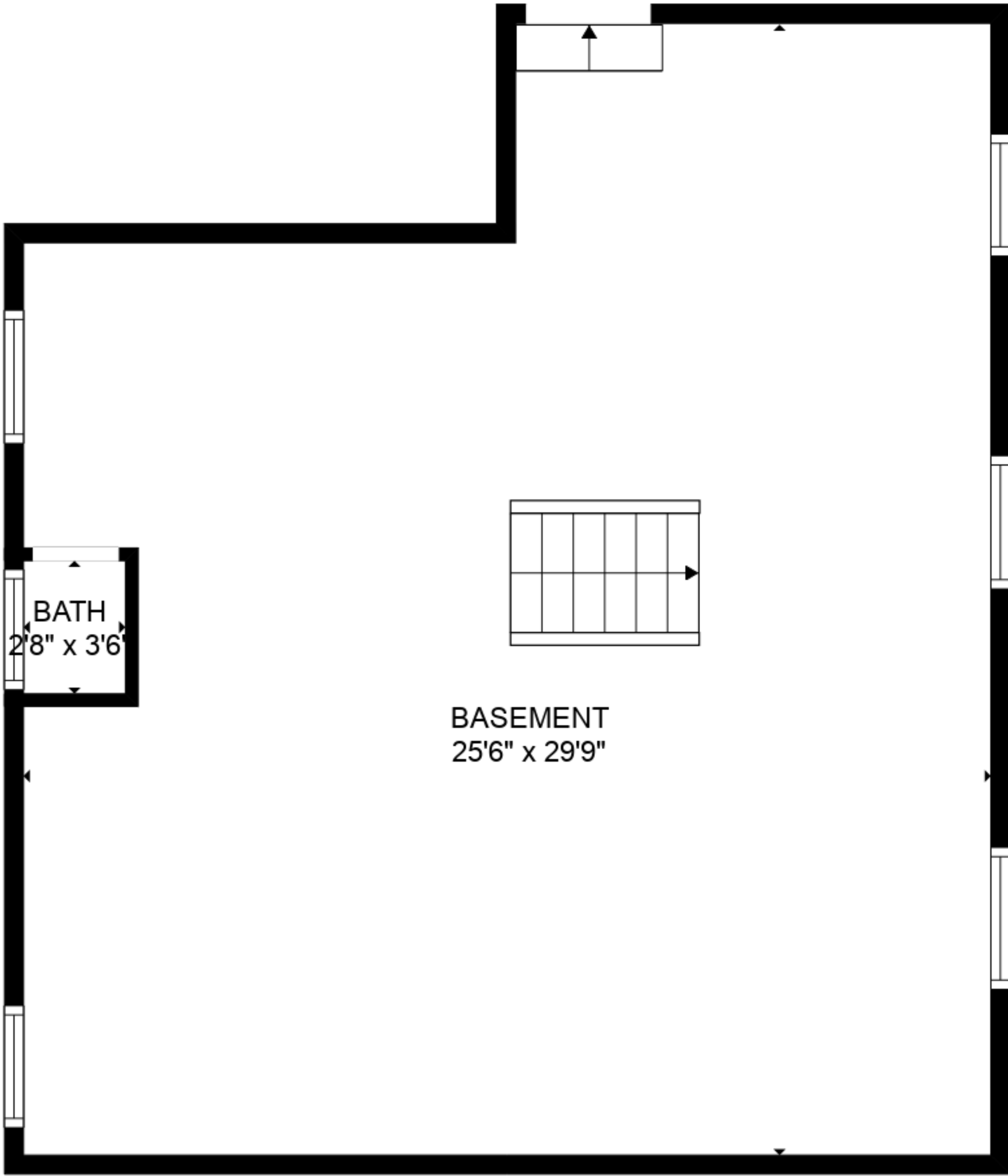
FLOOR 1
