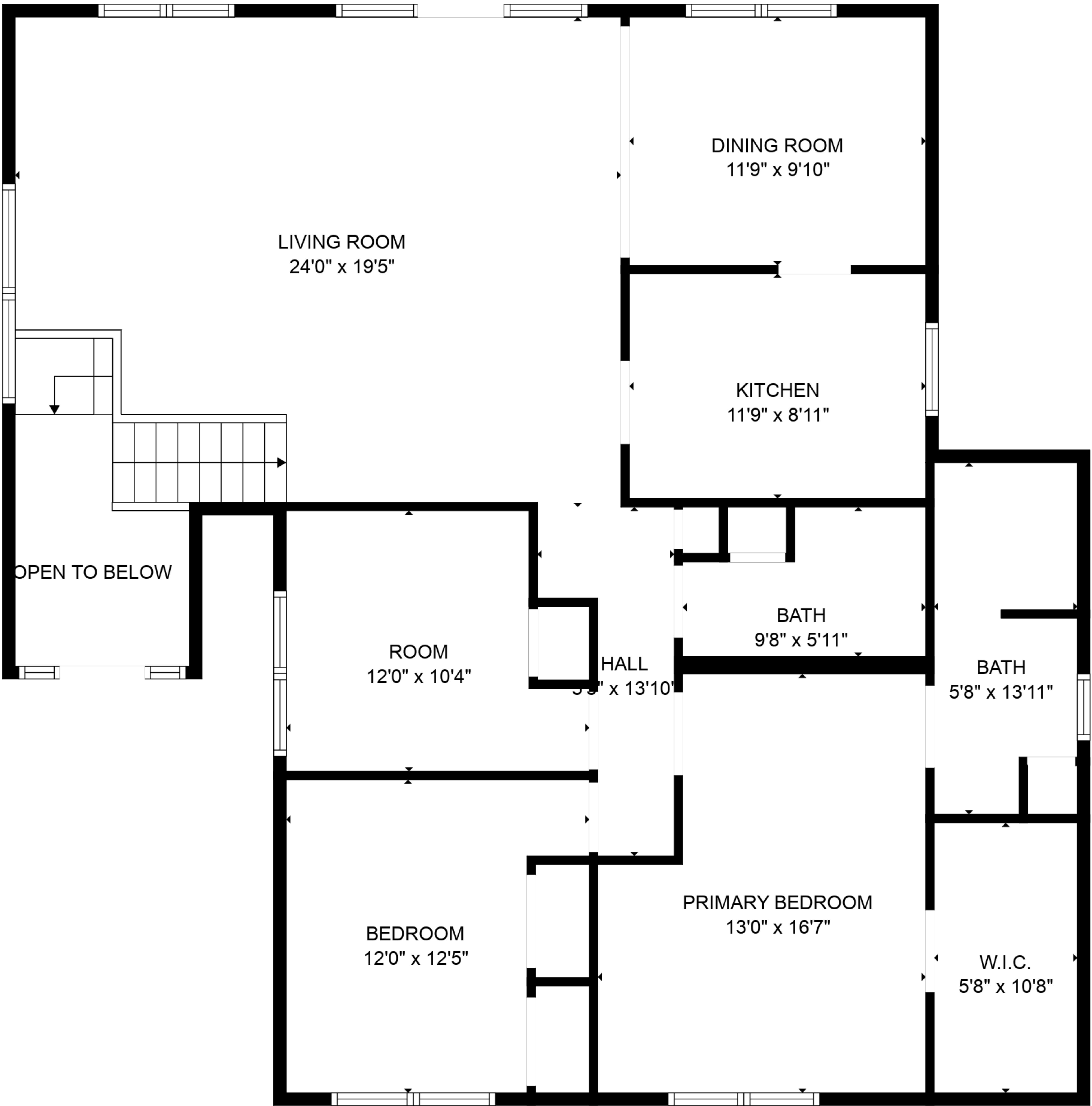
FLOOR 2
