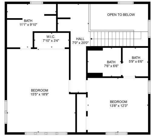
FLOOR 2
