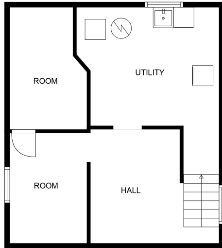
FLOOR 1
