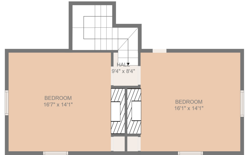
FLOOR 2
