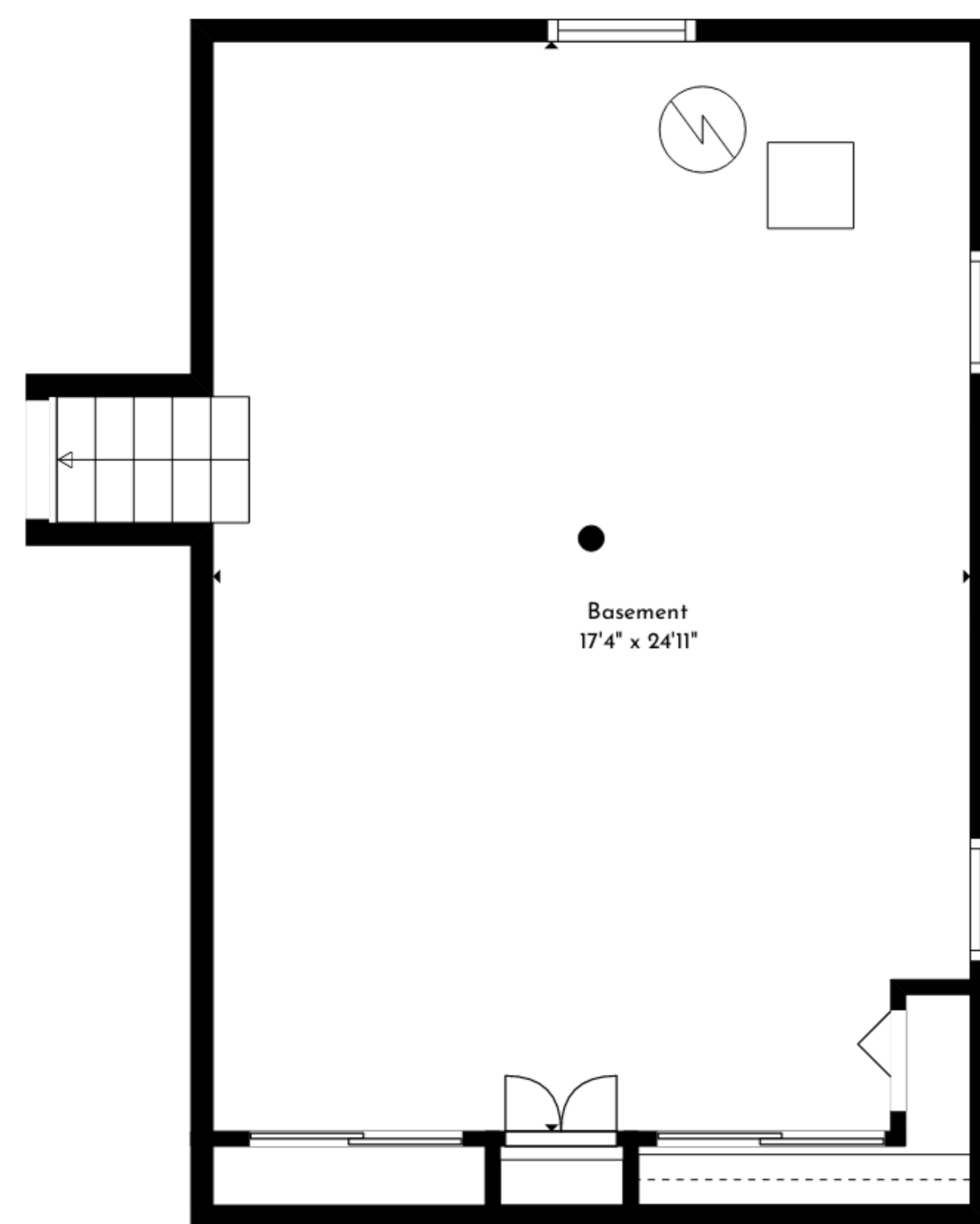
Floor 1
