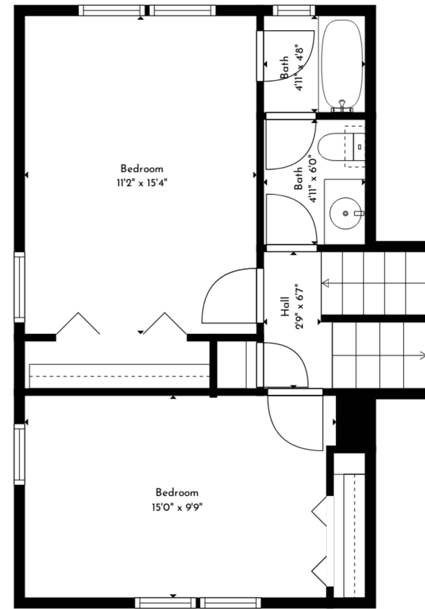
Floor 4
