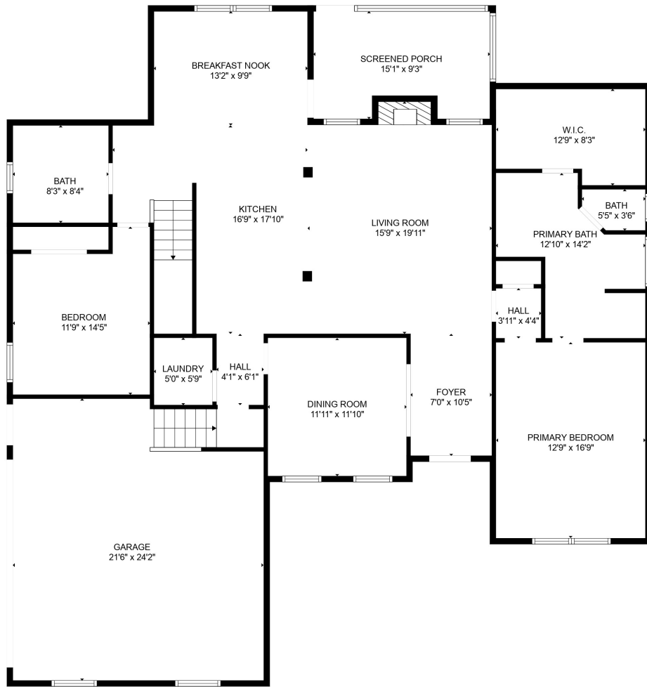
FLOOR 1
