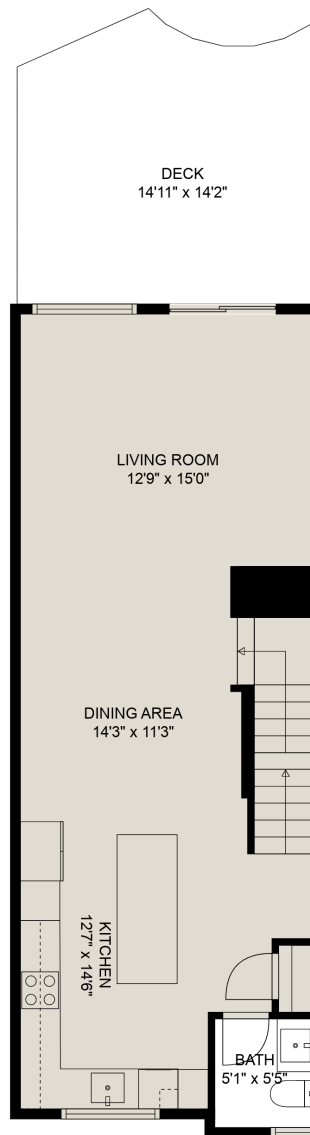
FLOOR 2
