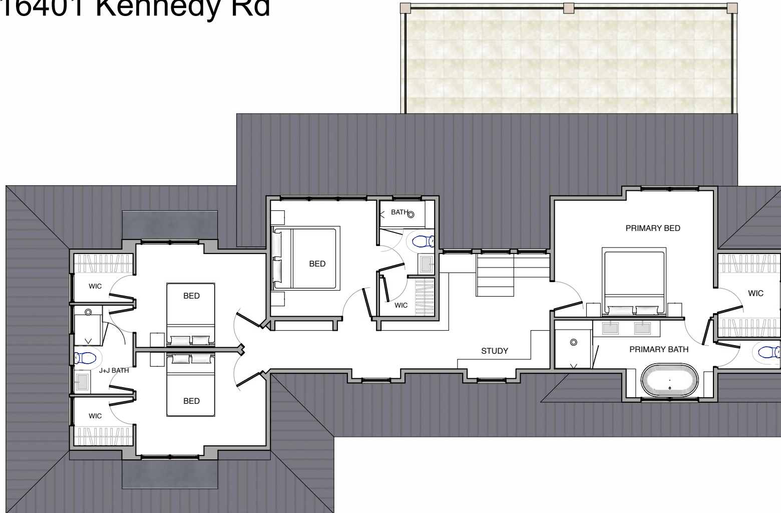
UPPER FLOOR PLAN 1370 sf
