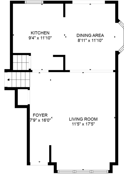
FLOOR 3
