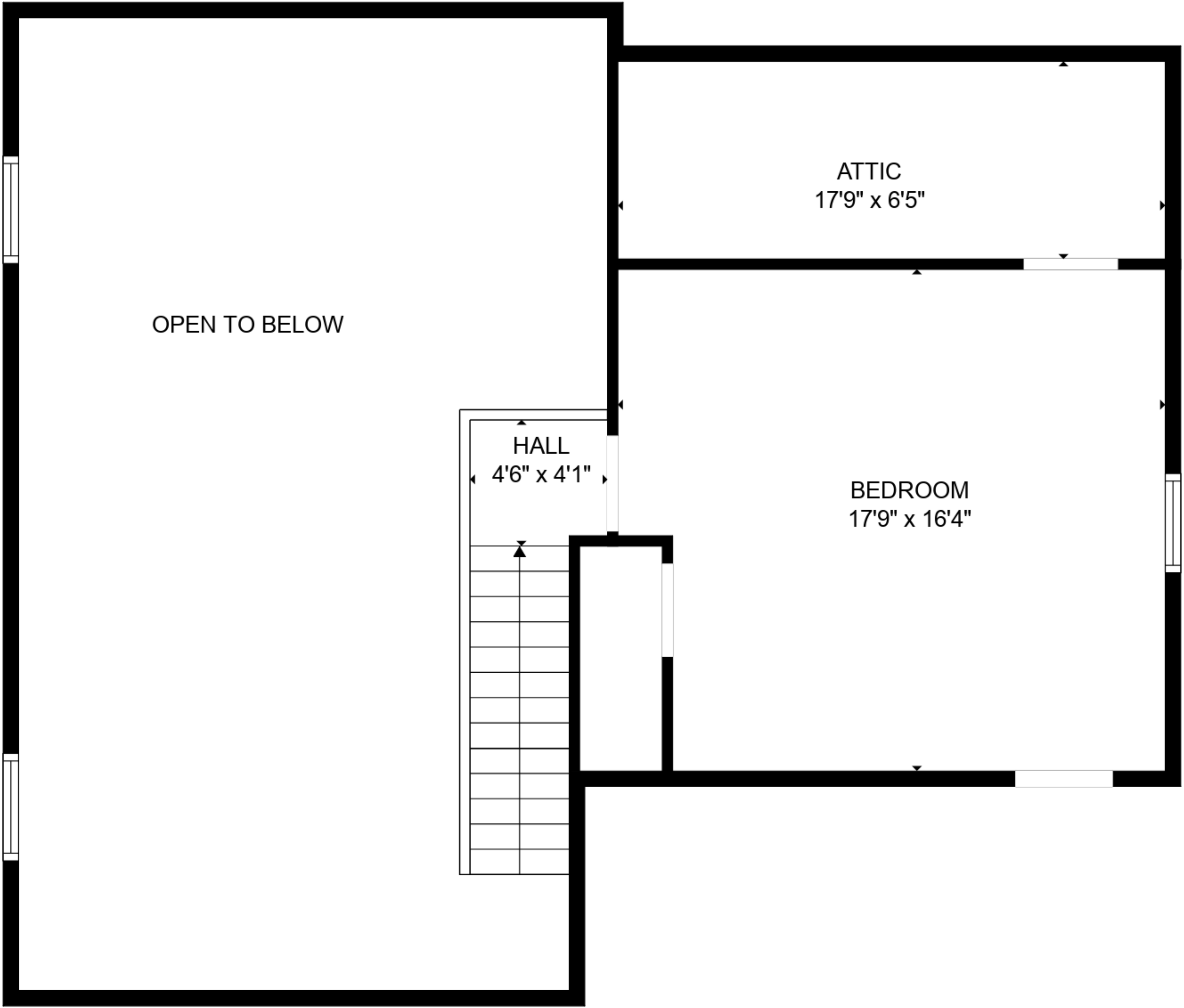
FLOOR 2
