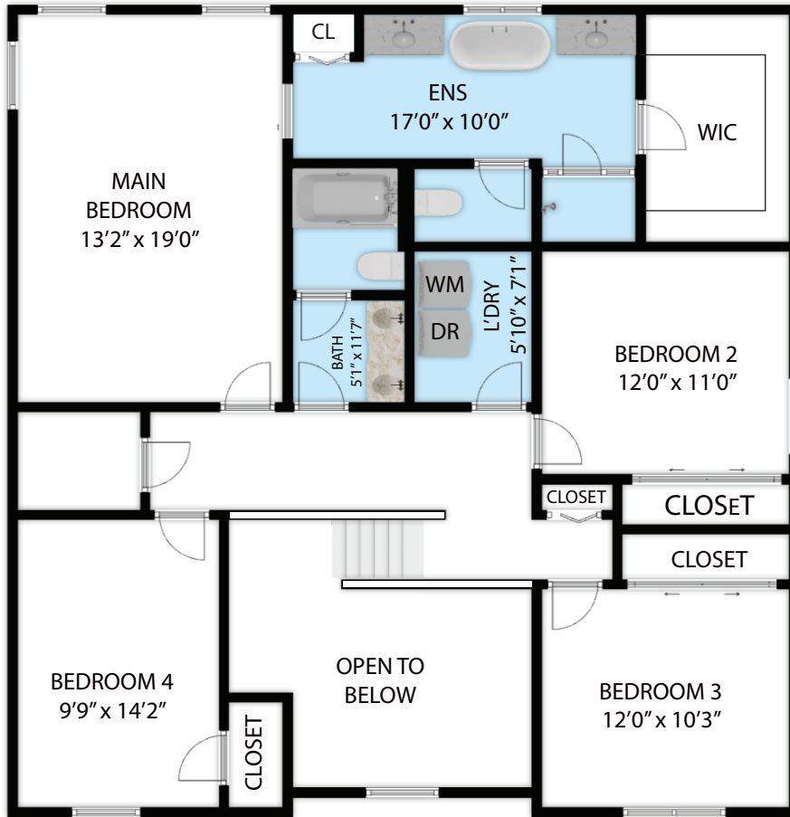
SECOND FLOOR
