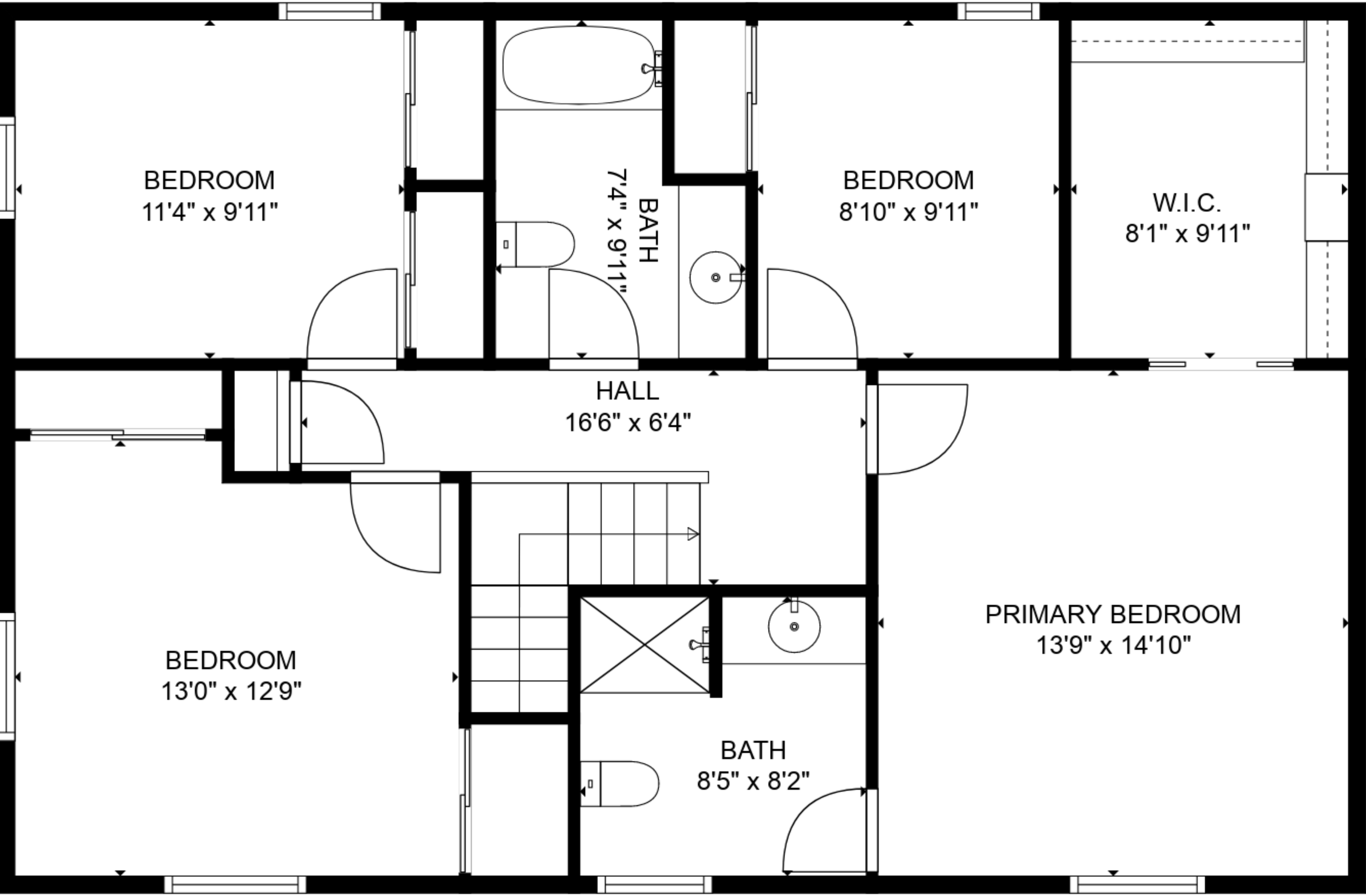
FLOOR 2
