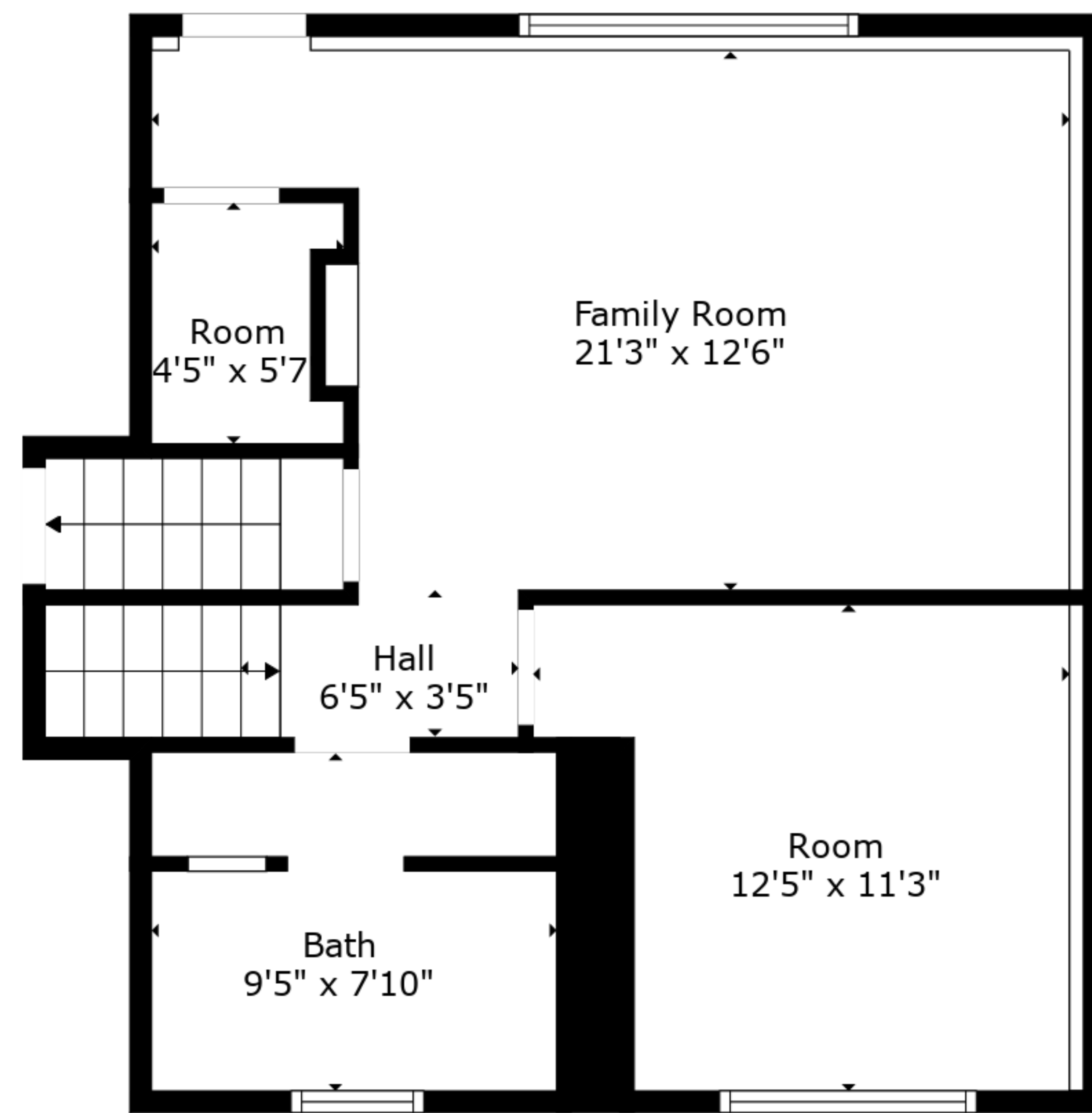
Floor 2
