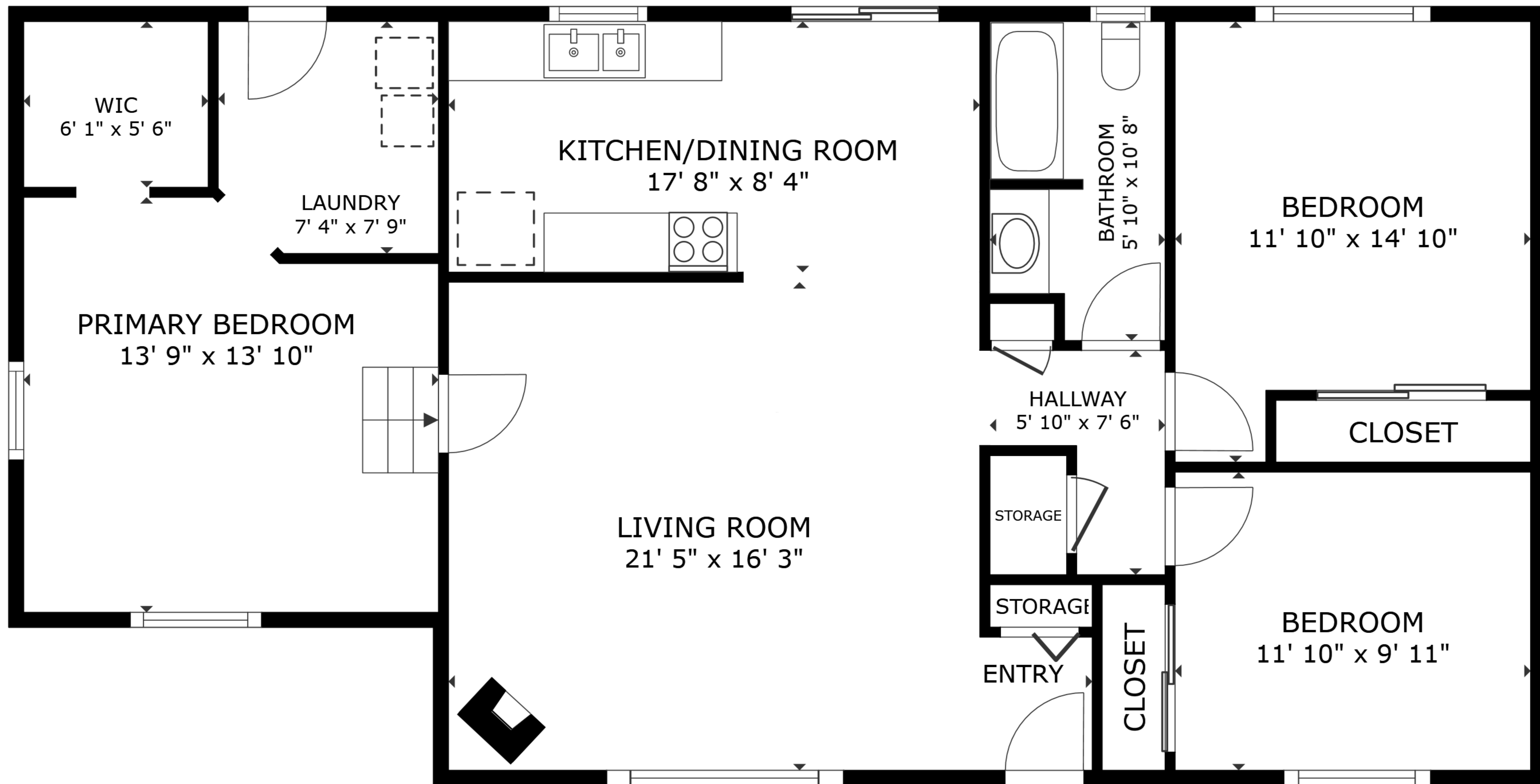
FLOOR PLAN
