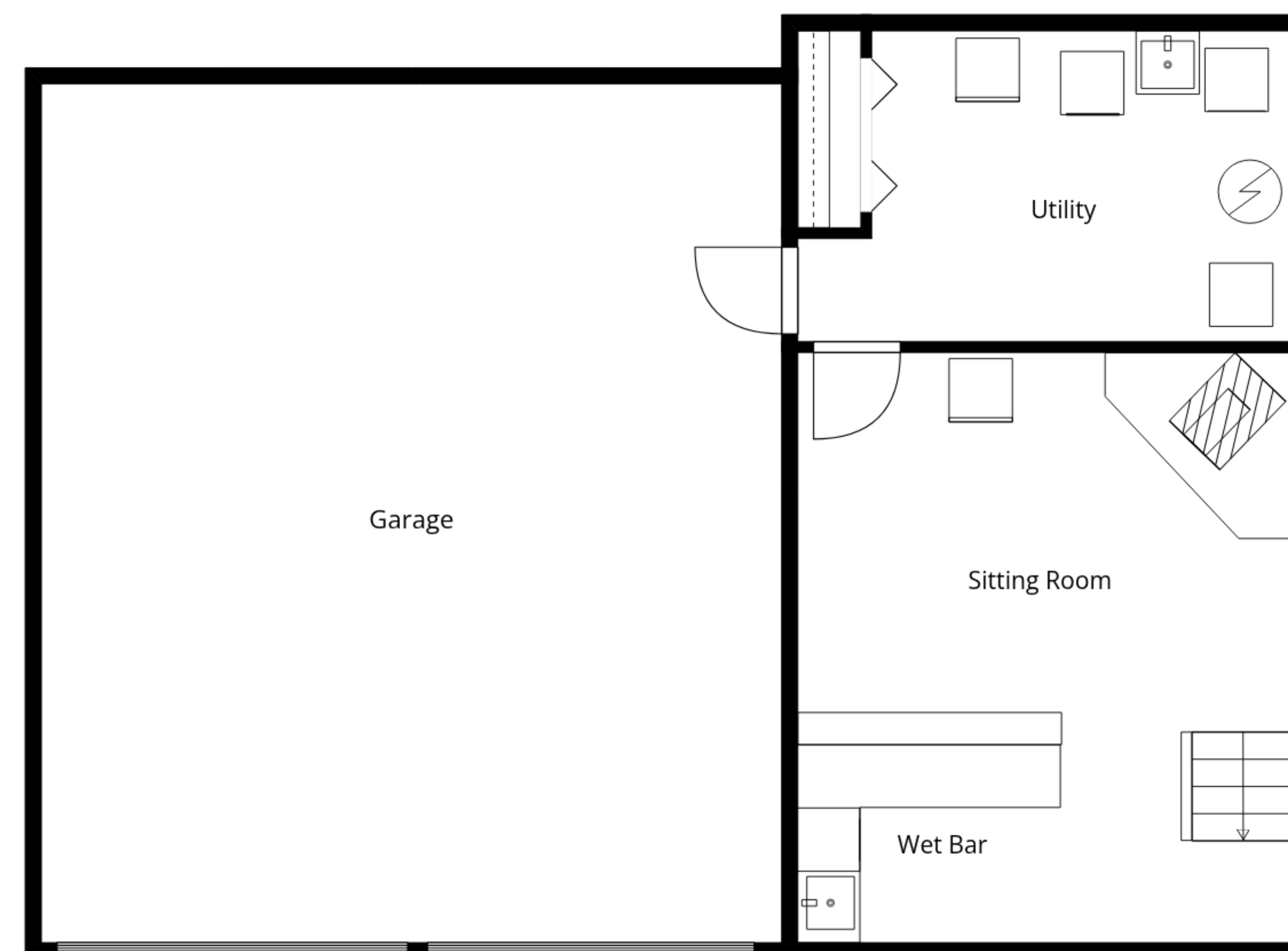
Basement 1
