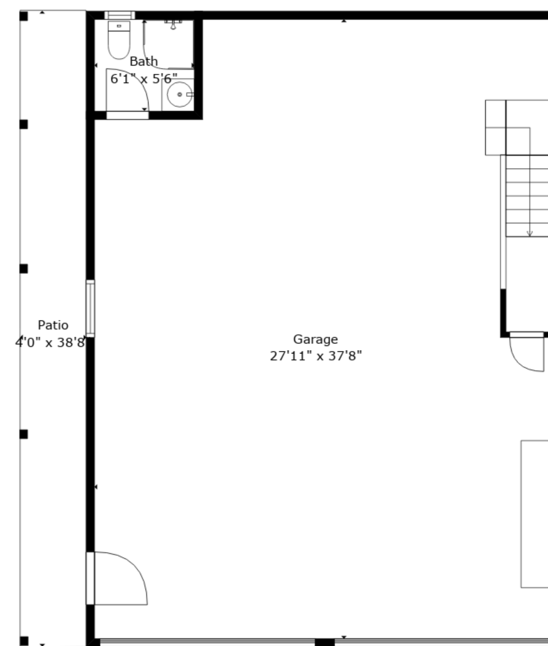
Floor 1
