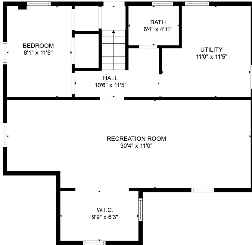
FLOOR 1
