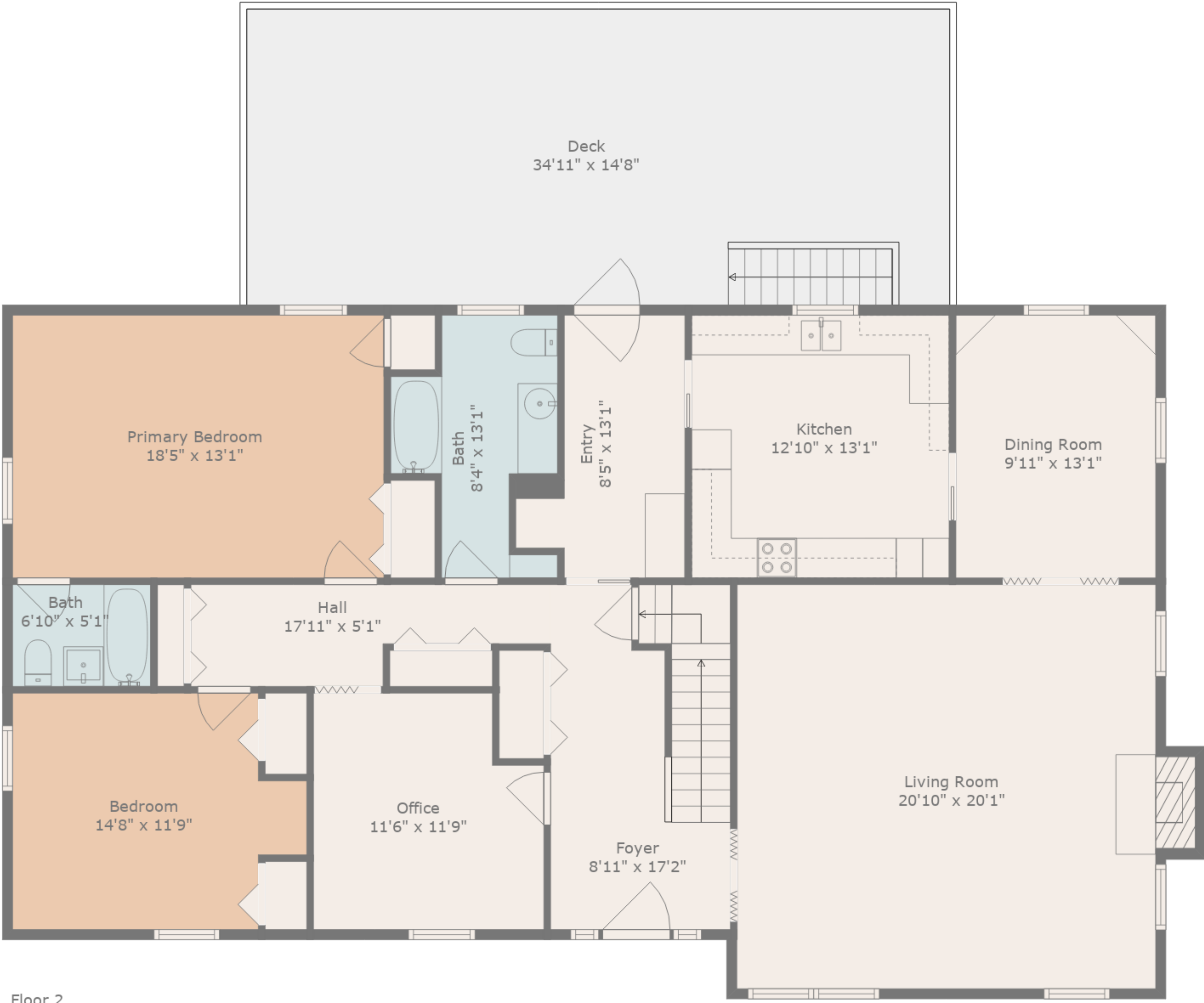
Floor 2
