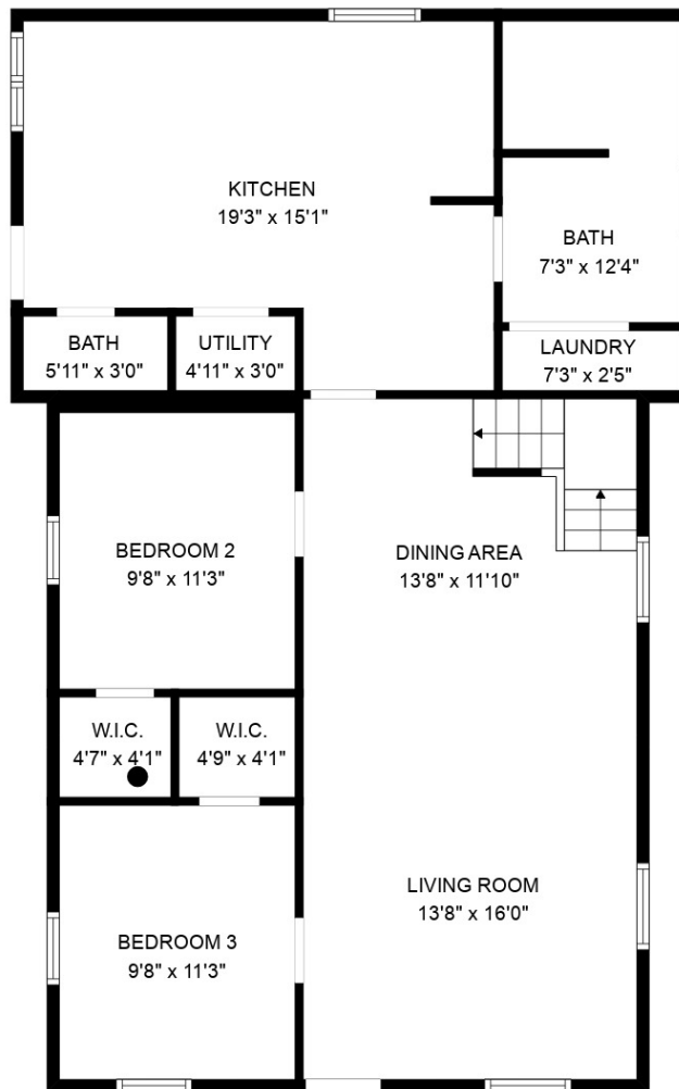
MAIN FLOOR
