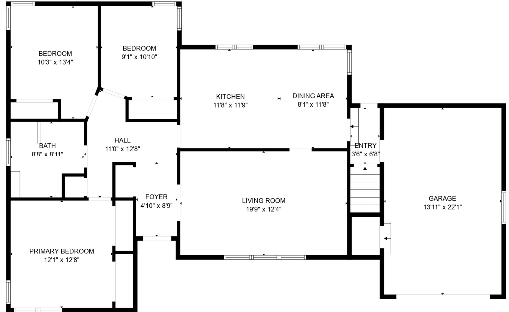
FLOOR 2
