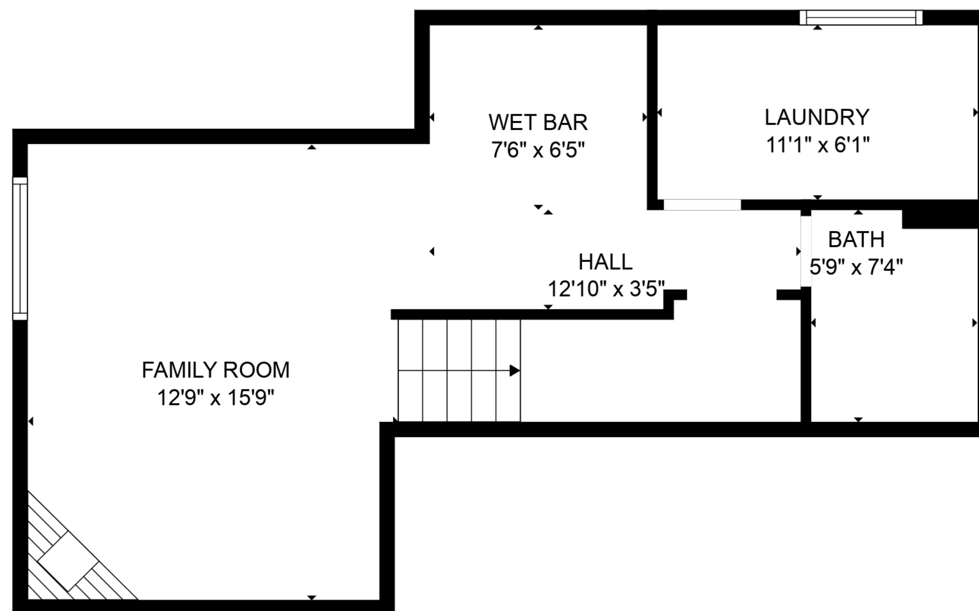
FLOOR 1
