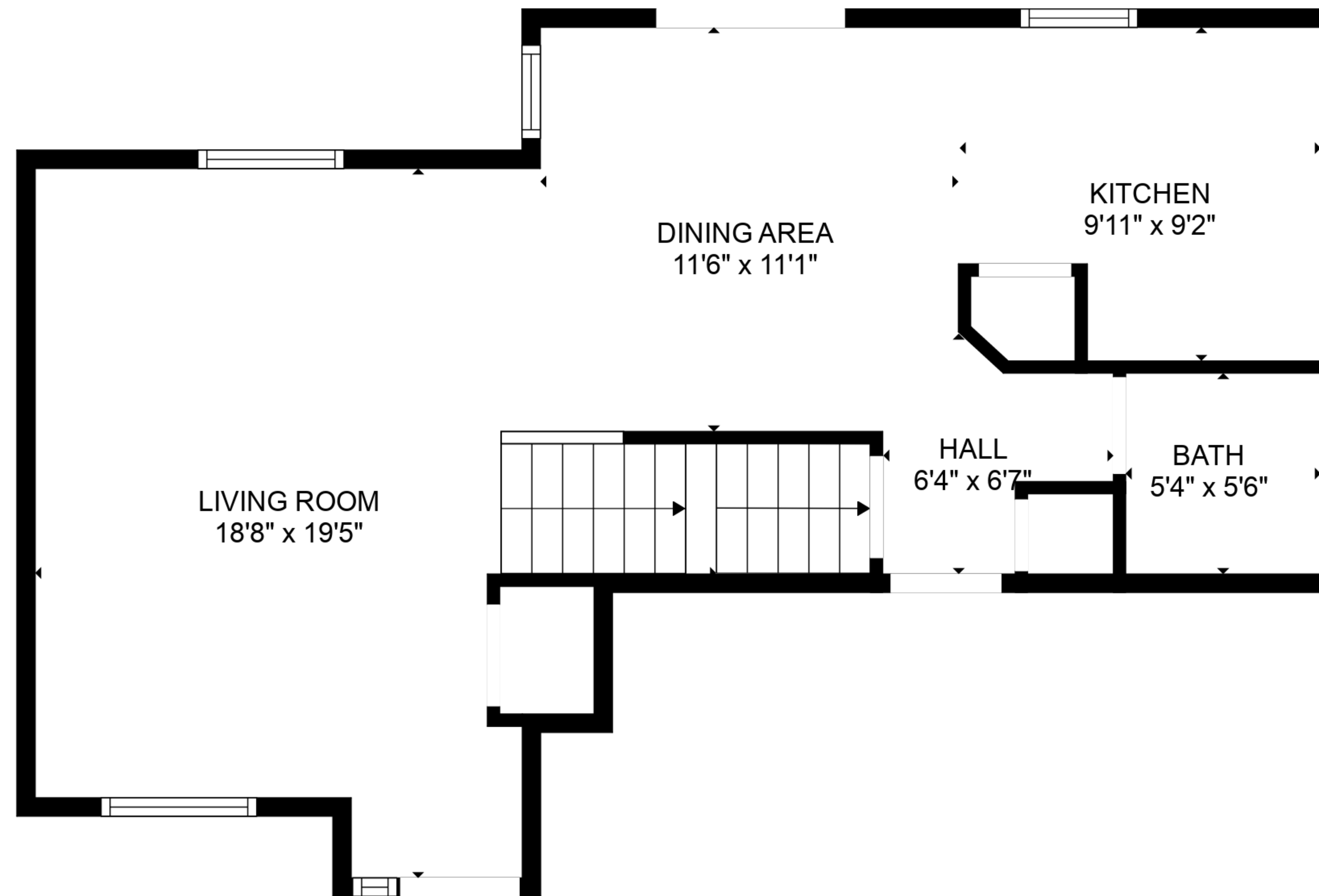
FLOOR 2
