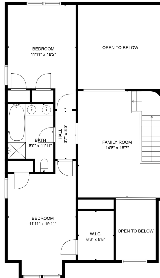
FLOOR 2
