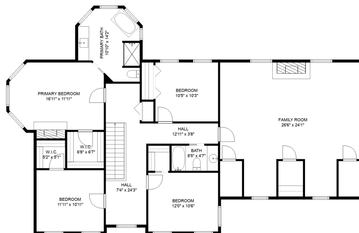
FLOOR 2
