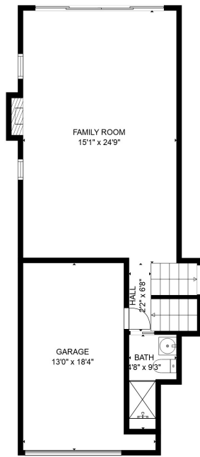
FLOOR 2
