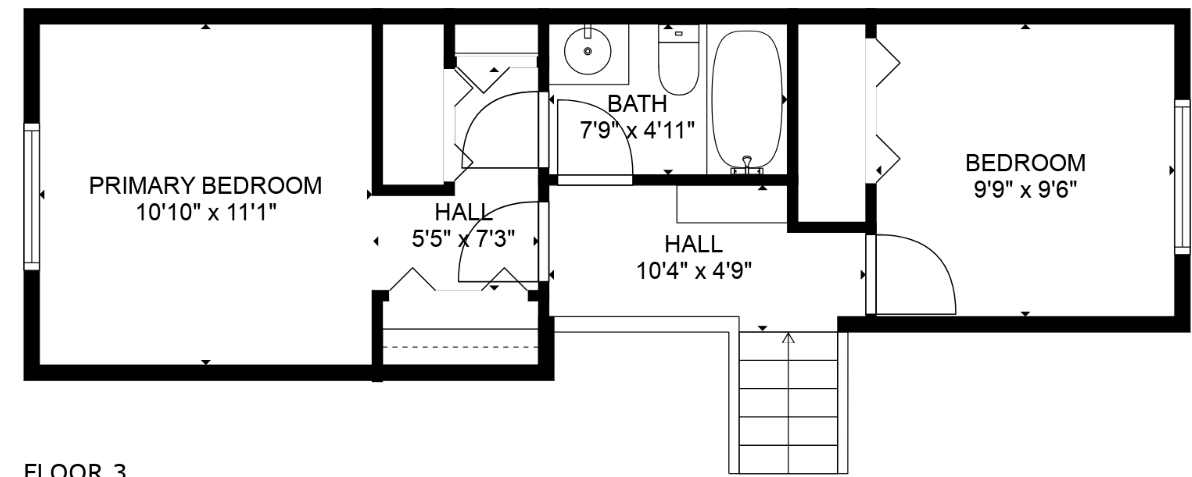
FLOOR 3
