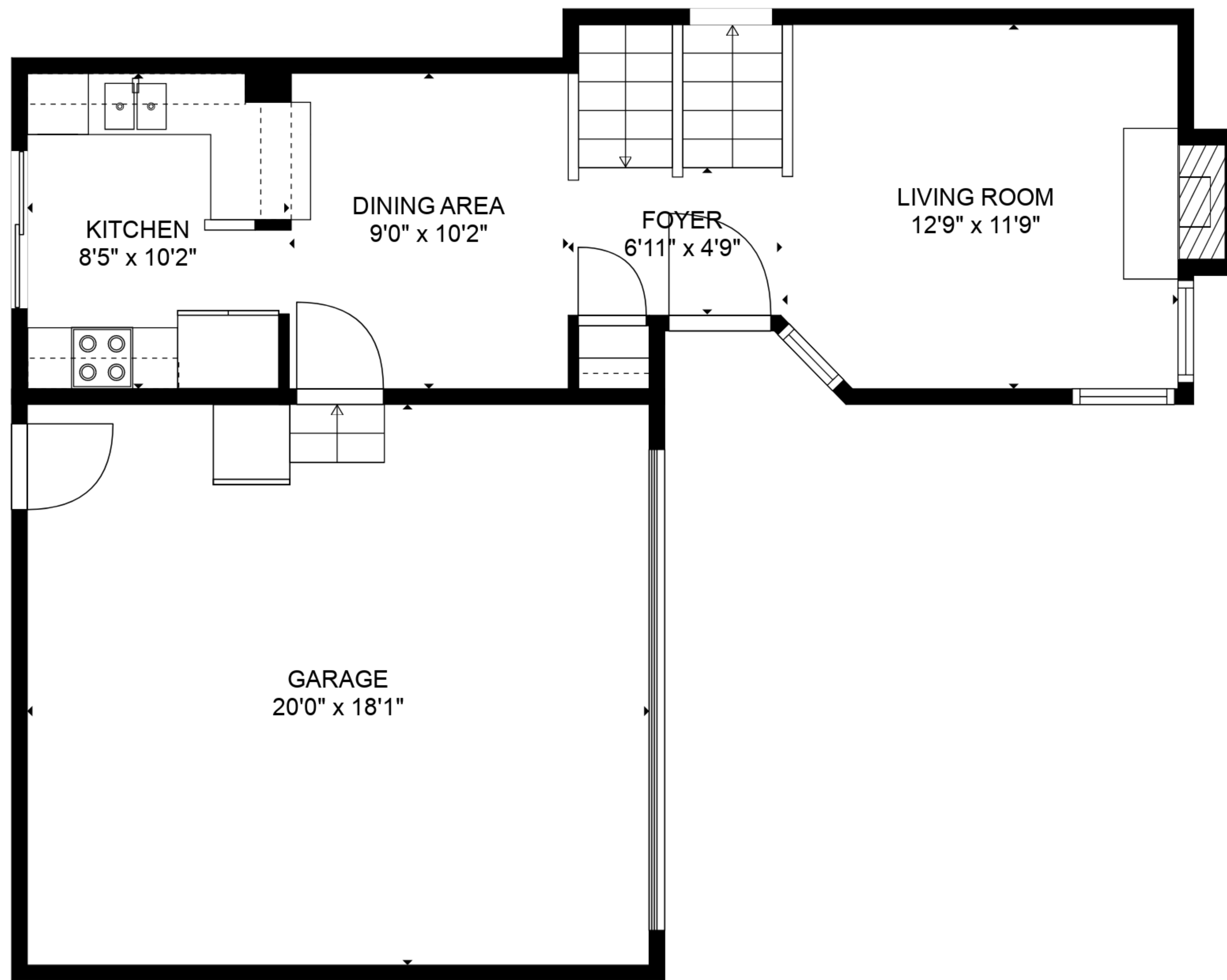
FLOOR 2
