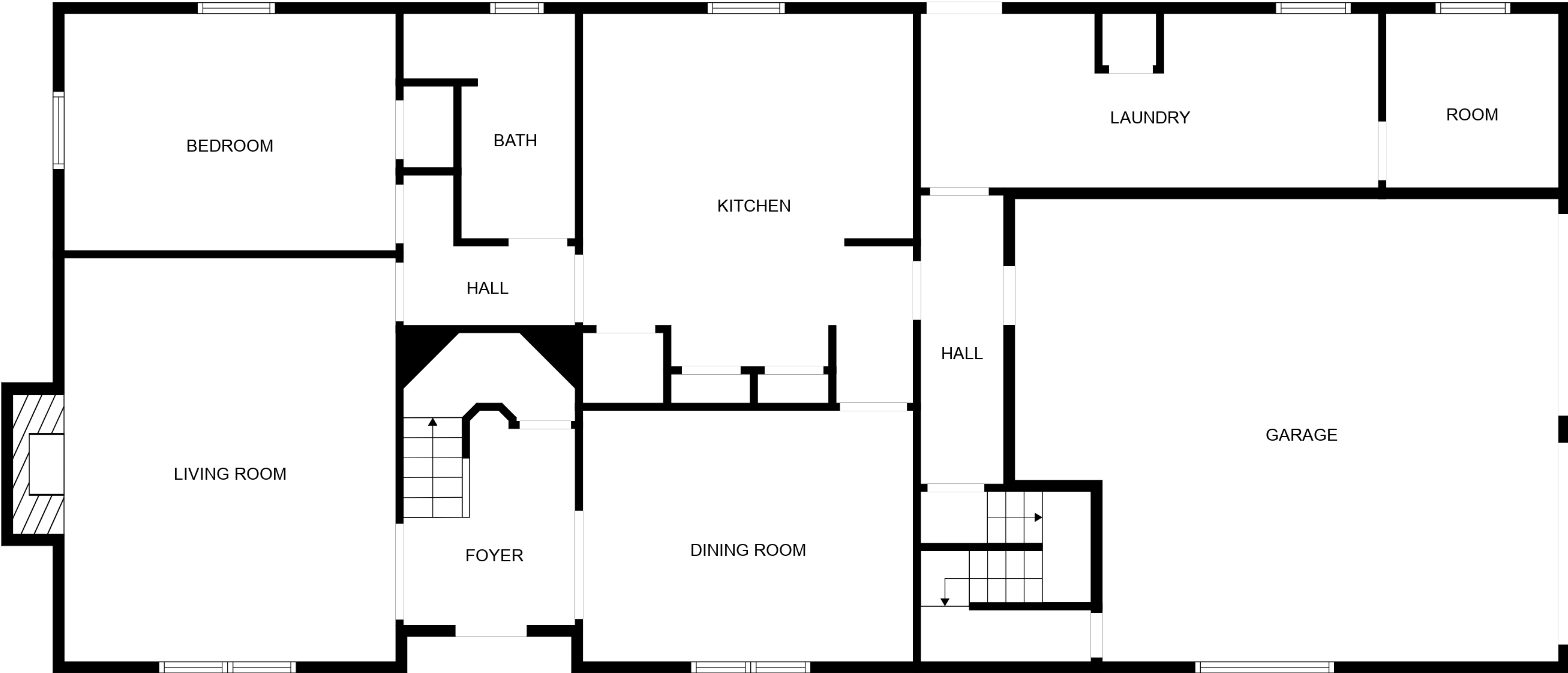
FLOOR 2
