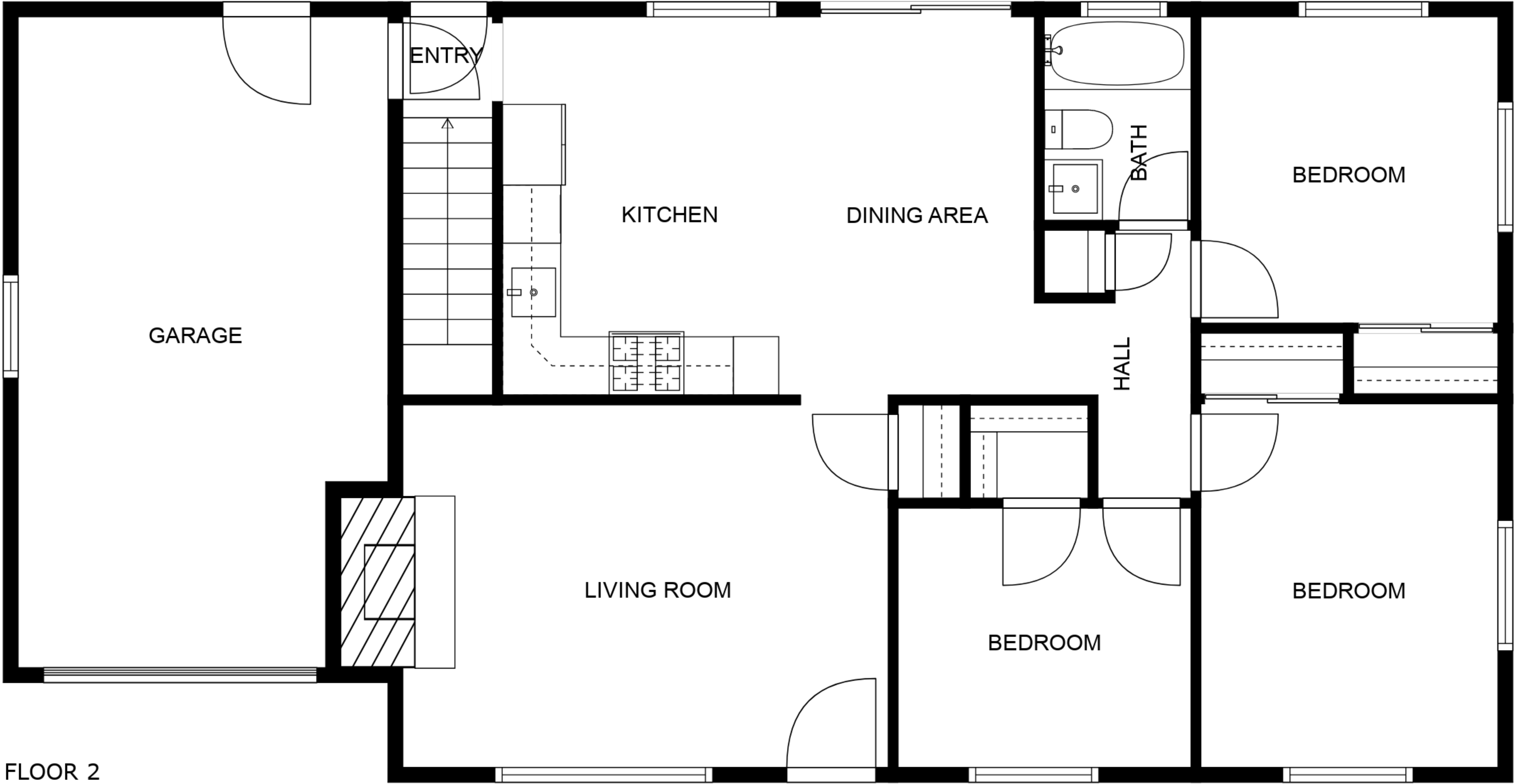
FLOOR 2
