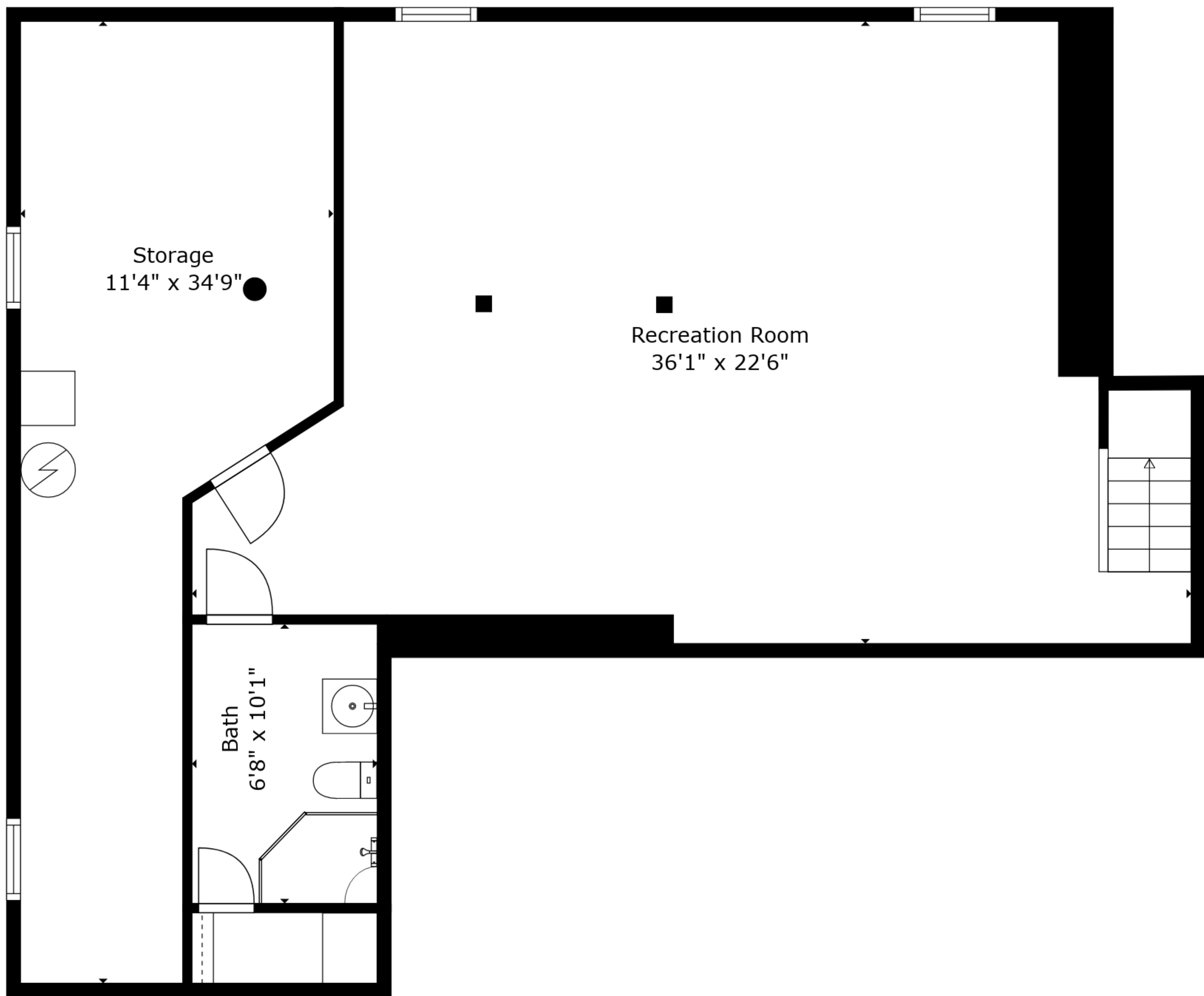
Floor 1
