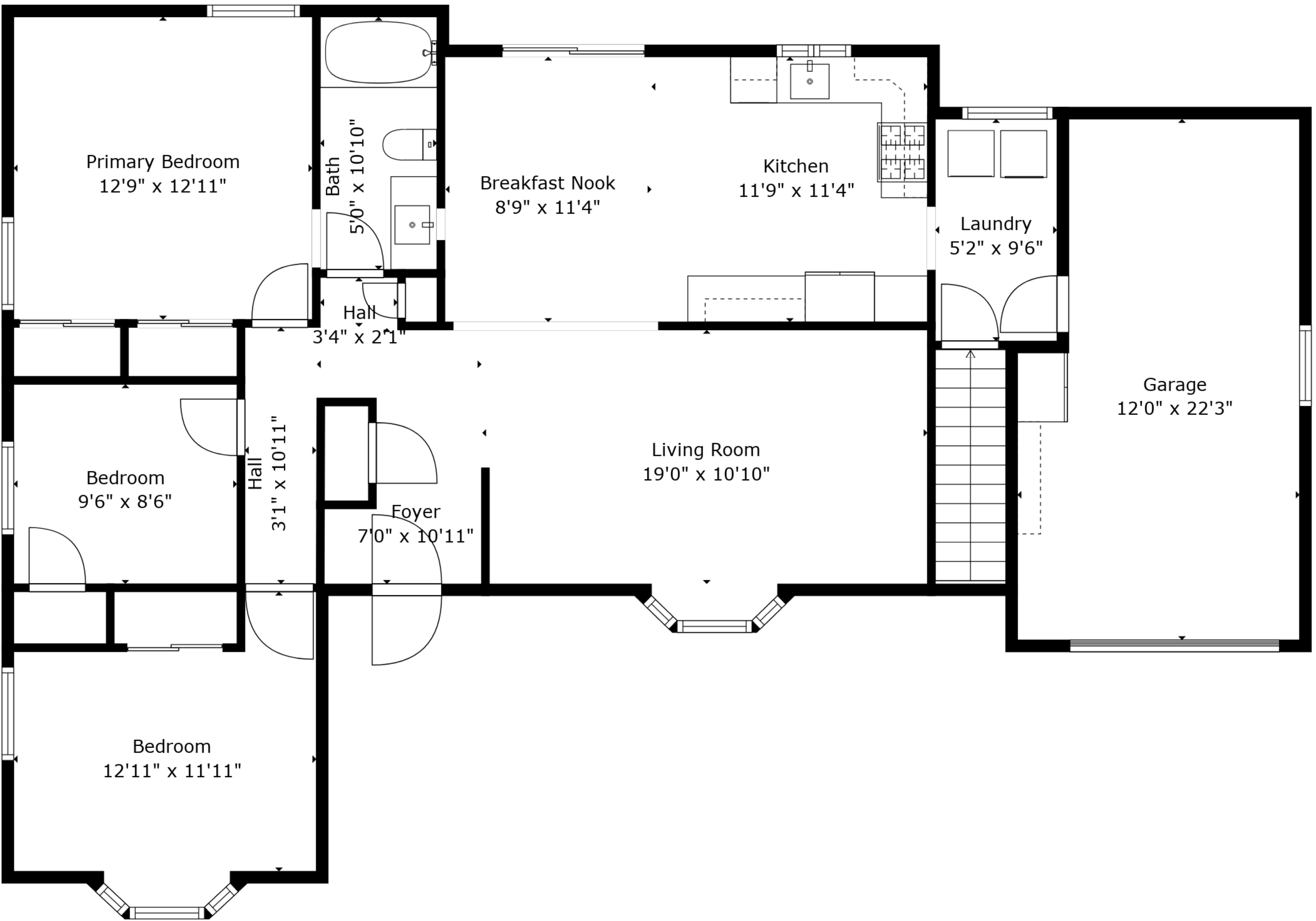
Floor 2
