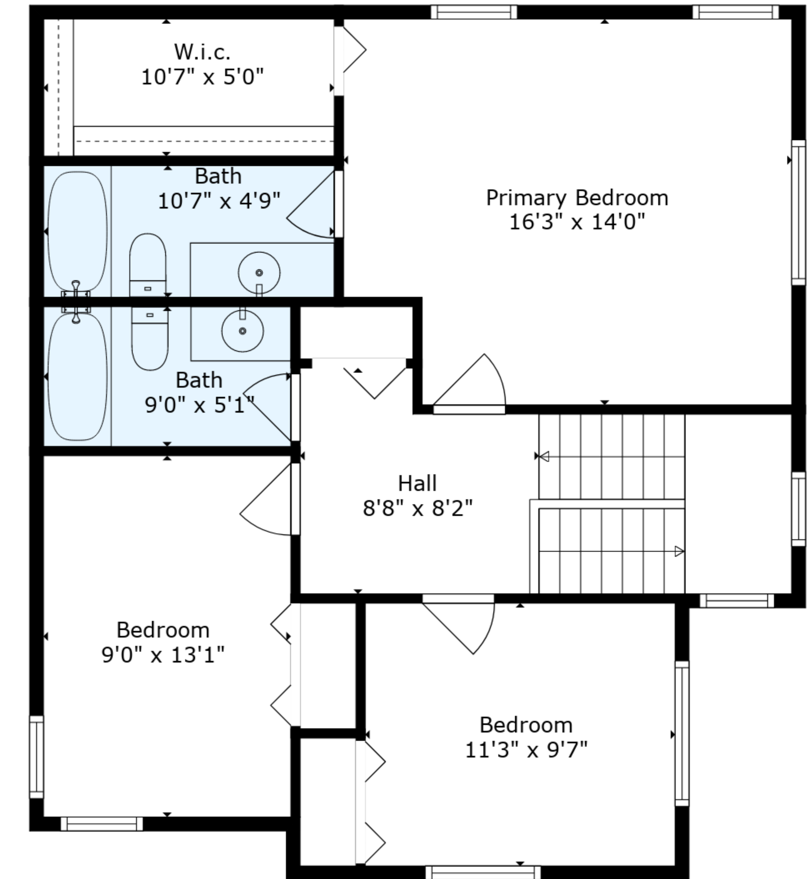
Floor 3
