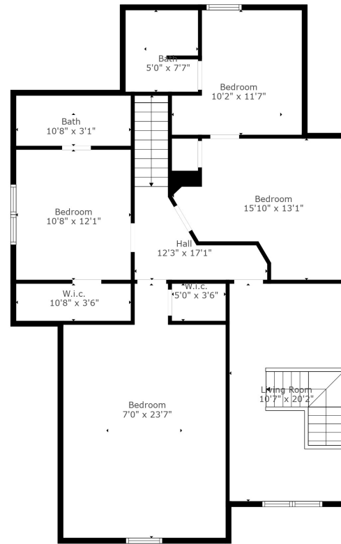
Floor 3
