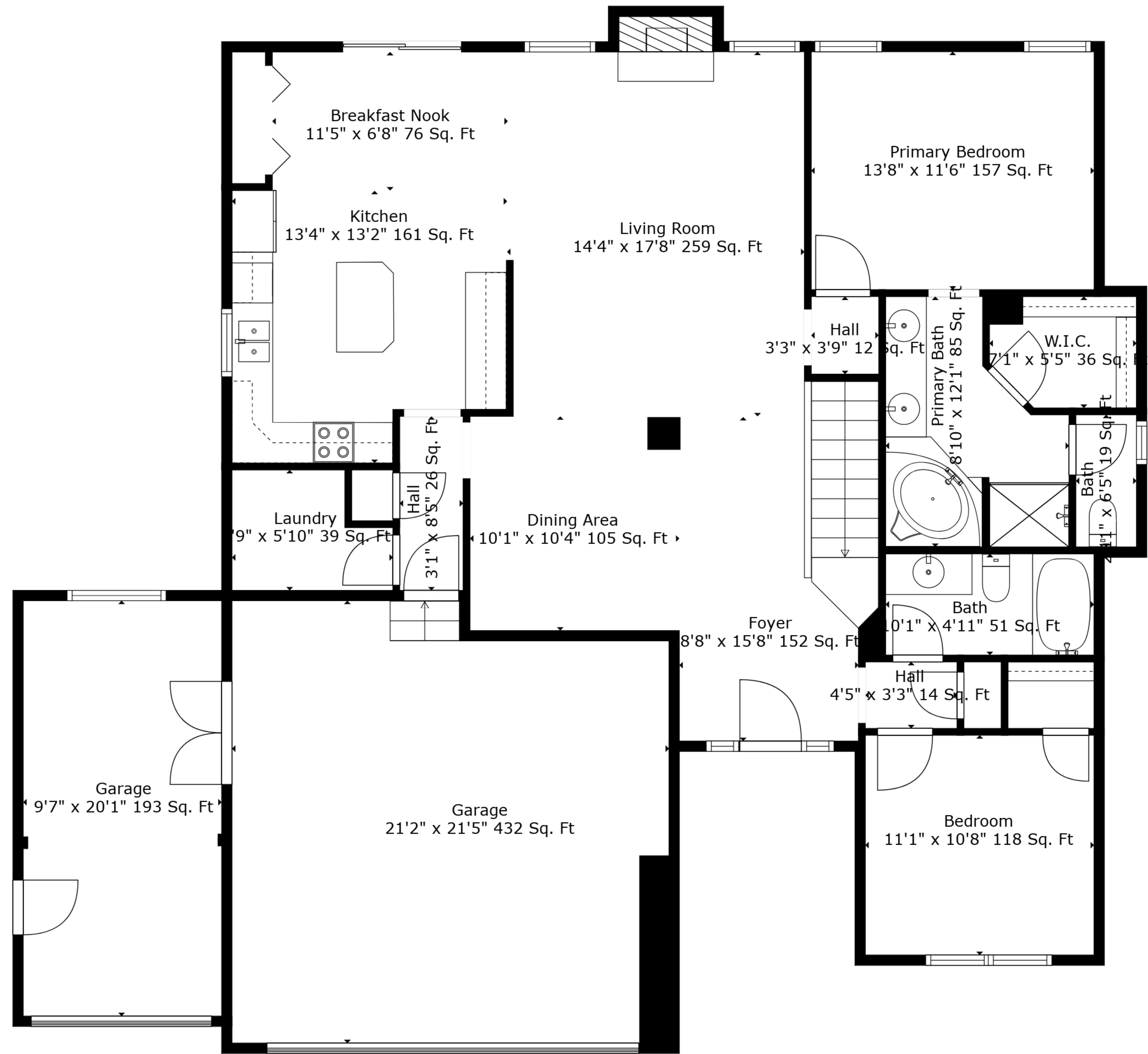
Floor 2
