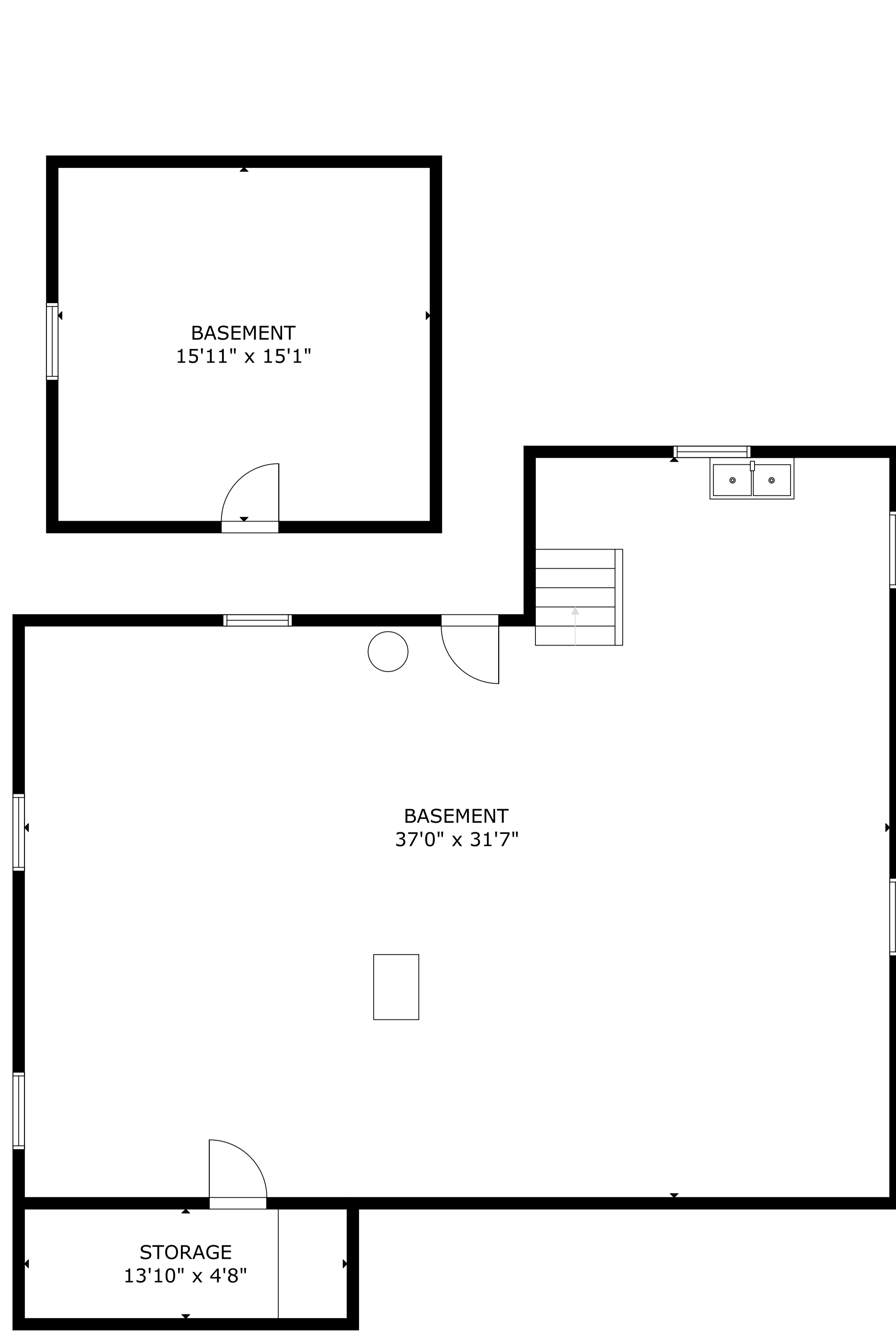
LOWER FLOOR
